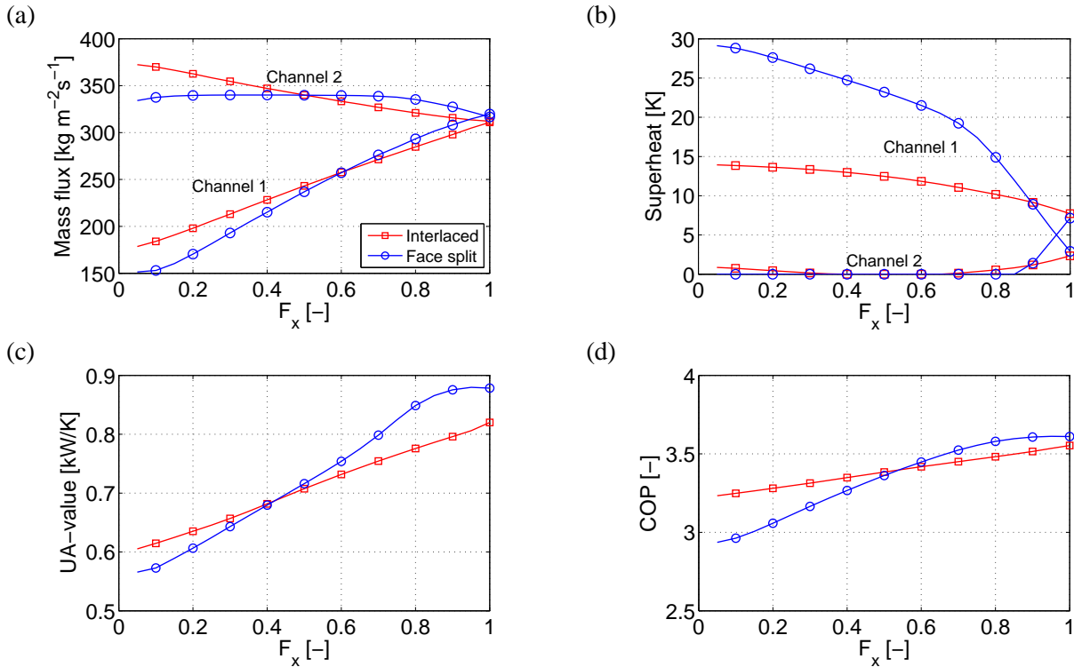
Figure 3. Selected parameters vs. the phase distribution parameter
