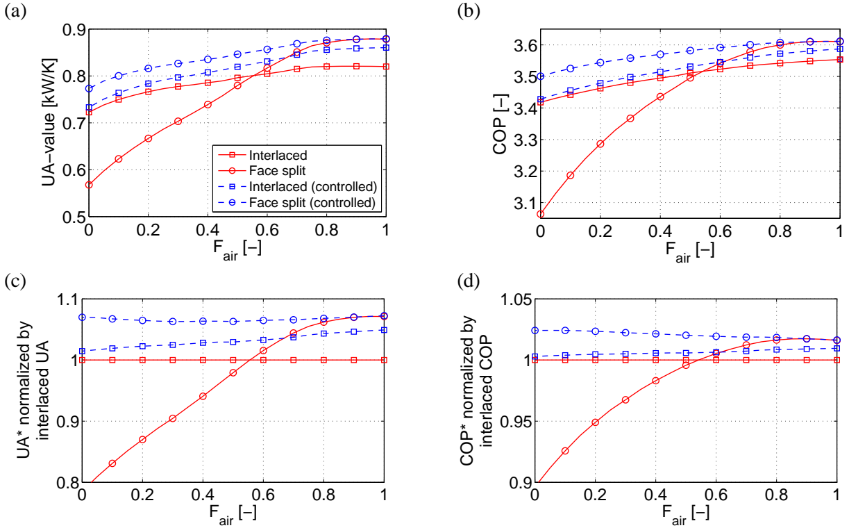
Figure 5. Comparison of UA-value and COP with/without compensation of airflow mal-distribution
