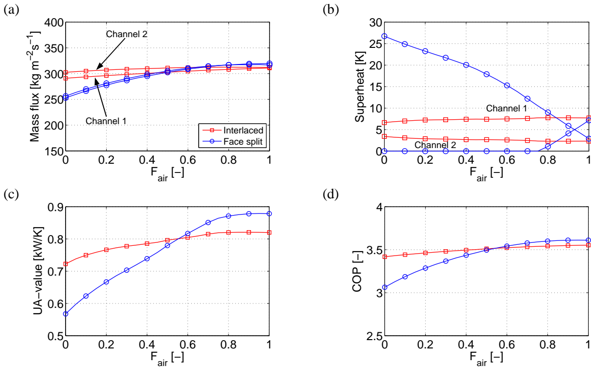
Figure 4. Selected parameters vs. the airflow distribution parameter
