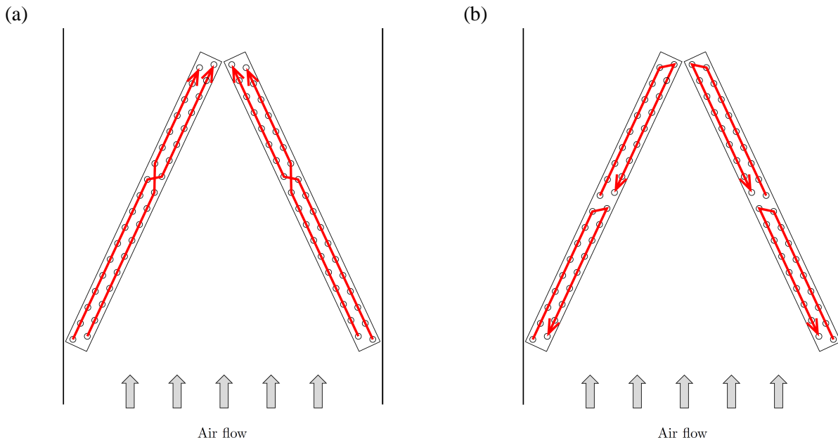
Figure 1. Tube circuitries of (a) the interlaced evaporator and (b) the face split evaporator
