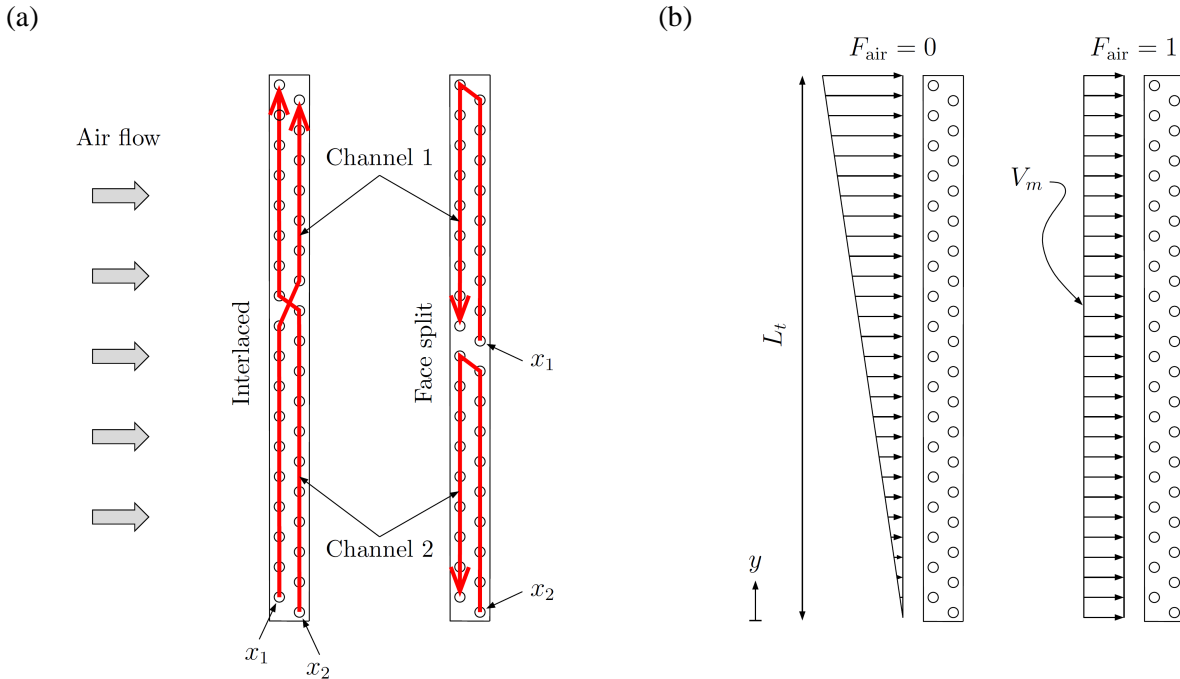
Figure 2. (a) channel numbering for each evaporator and (b) one-dimensional airflow profiles
