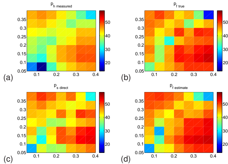
Figure 4 – SPL at 500 Hz of the primary source radiating in the presence of a reflecting panel. (a) Measured pressure in the hologram plane. (b) Measured free field pressure in the reconstruction plane. (c) Reconstruction with the direct formulation, equation (4) . (d) Estimation of the free field pressure with equation (17)
