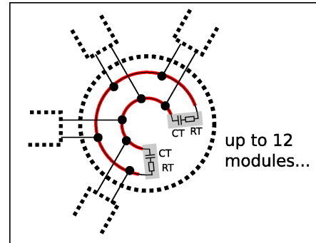
Fig. 6. Local buses of Odin. One AC termination is placed at each end of the bus. The maximum number of modules to be connected to the local bus is 12, and each module contributes 1/8 of load to the bus. The value of the capacitor C_T of the AC termination is determined by the maximum expected length of the hybrid buses (not the length of the local buses).
