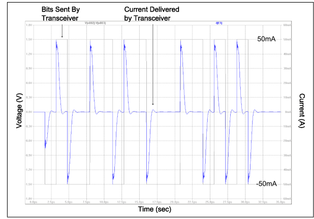
Fig. 11. Current being delivered or received by one of the differential outputs of the modeled transceiver. The current is positive and negative, but is always provided by the same same transceiver (from alternated differential outputs). The peaks achieved are within the capabilities of commercial transceivers.
