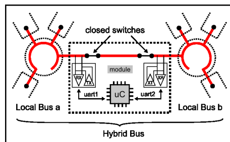
Fig. 3. A module merging two local buses into a more global bus (hybrid bus) by closing its internal switches. If another adjacent module also closes its switches, the hybrid bus grows. When the hybrid bus is able to communicate all the modules within the system, it becomes a global bus. Here, the buses are represented by a single line, in spite of they are conformed by two wires.
