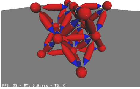
Fig. 7. CCP lattice arrangement of Odin. If we continue expanding the size of the arrangement, by attaching more modules to the joints, the average number of modules per joints will converge to 12. The image was taken from the USSR simulator (Unified Simulator for Self-Reconfigurable Robots), which includes a model of the Odin system.
