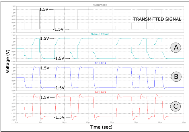
Fig. 10. Digital signal ideally transmitted, and then sampled at one extreme of each local bus: A, B, and C. The non-ideal AC termination produces reflexions, which are successfully damped before the pulses end. The maximum trip delay is the time required for a signal to travel 16 meters in twisted pair cable. In the hybrid approach, the bit width is 20 times the maximum trip delay, and the time constant \tau = R_T C_T , is 2 times the maximum trip delay.
