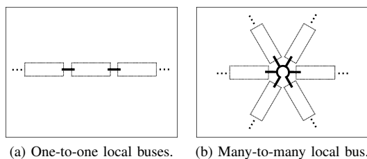
Fig. 2. Different types of local buses. Here, modules are represented by rectangles and buses by lines. In (a), the local buses connect two adjacent modules (neighbour-to neighbour communication). An example of this kind of system is homogeneous modular chain-type self-reconfigurable robots. In (b), a local bus connects many adjacent modules. In this kind of system, the local buses may be implemented outside the modules, within special types of modules acting as joints. An example of this kind of system is heterogeneous modular lattice-type self-reconfigurable robots.
