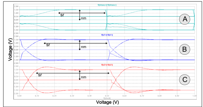
Fig. 12. Eye Pattern of the Spice simulation. The digital signals are sampled at one extreme of each local bus: A, B and C, but now against an appropriate synchronizing clock signal (not time in the horizontal axes). The bigger the distances nm and sr (or the more open the eye), the better the quality of the signal.
