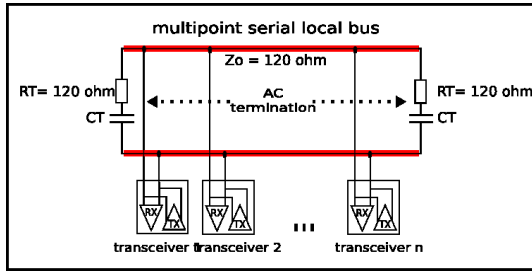
Fig. 4. A local bus implemented using a transmission line with characteristic impedance Z_0 = 120\Omega . The AC termination consist of one resistor R_T in series with one capacitor C_T . R_T matches the characteristic impedance of the line, Z_0 = 120\Omega , and C_T is dependant on the expected maximum length of the hybrid buses. The AC termination is a balance between signal quality, power requirement, and transmission rates.
