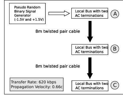
Fig. 9. Block Diagram of the Spice Simulation. The Pseudo Random Binary Signal Generator (PRBS) information is coupled directly to the first local bus (A); then it is forwarded to the second local bus (B), which is connected by 8 meters of cable; and finally, it is forwarded to the third local bus (C), which is connected by 16 meters of cable (8+8 meters).
