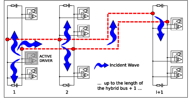
Fig. 8. Example of topology created by hybrid buses. The transceiver acting as driver is coloured grey and the incident wave (not the reflexions) of the digital information is drawn with thick curly arrows. The active transceiver is driving more than one bus (AC terminated), and the local buses may be joined at other points than the extremes or the middle.
