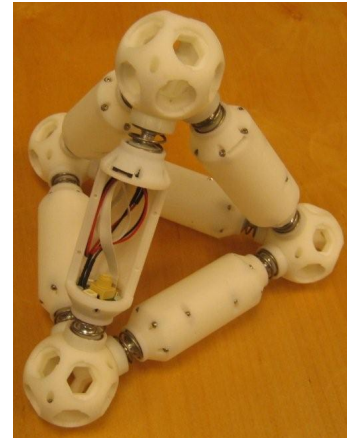
Fig. 5. First prototype of the novel Odin modular robot. In the Odin robot, modules are connected to joints (balls) to form a robot configuration. Here we can see 4 joints shaping 6 modules into a tetrahedron, a sub arrangement of the cubic close packing lattice (CCP). The joints wrap local buses, the modules embed the extending bus, and the connectors forward the electrical connections. The diameter of the joints is 50mm and the length of the modules is 110mm.
