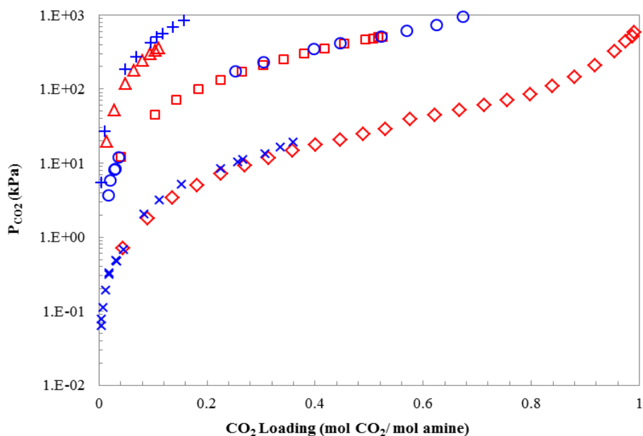
Figure 1: VLE of CO 2 with 5M DEEA at 40, 80 and 120°C. This work: \diamond , 40°C; \square , 80°C and \Delta , 120°C. Monteiro et al. [6]: \times , 40°C; \circ , 80°C and + , 120°C.
