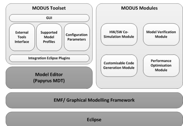
Figure 6: MODUS toolset integration architecture
