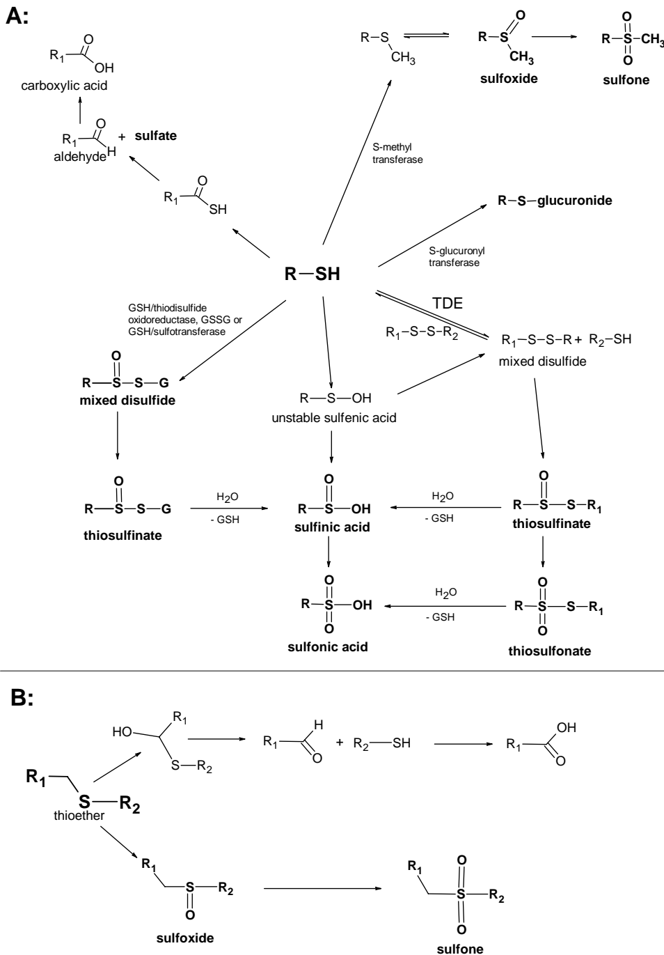
Figure III.3 Metabolism of organic sulphur compounds. A panel: metabolism of thiols and disulphides. B panel: metabolism of thioethers. Structures in bold are major excretion products. TDE = Thiol-Disulphide Exchange
