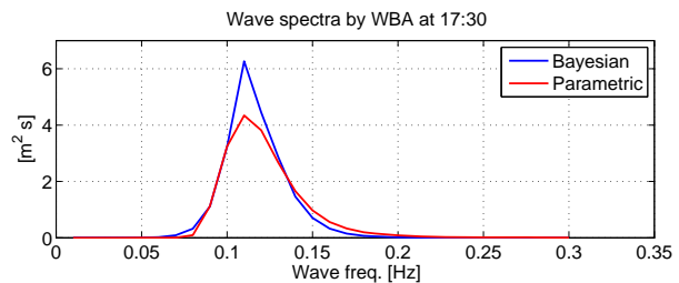
Fig. 7: The legend is identical in all plots. NB. the Radac system cannot not estimate wave heading.
