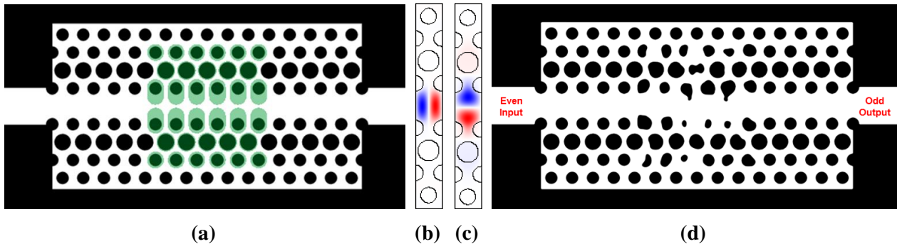
Fig. 1. (a) Initial design of the PhCW defined by air holes (black) arranged in a triangular lattice in silicon (white). Also shown is the design domain (green) chosen in the TO. 2D mode plots for the (b) TE 0 and (c) TE 1 mode of the PhCW. (d) Topology optimized mode converter design obtained by utilizing 2D TO.
