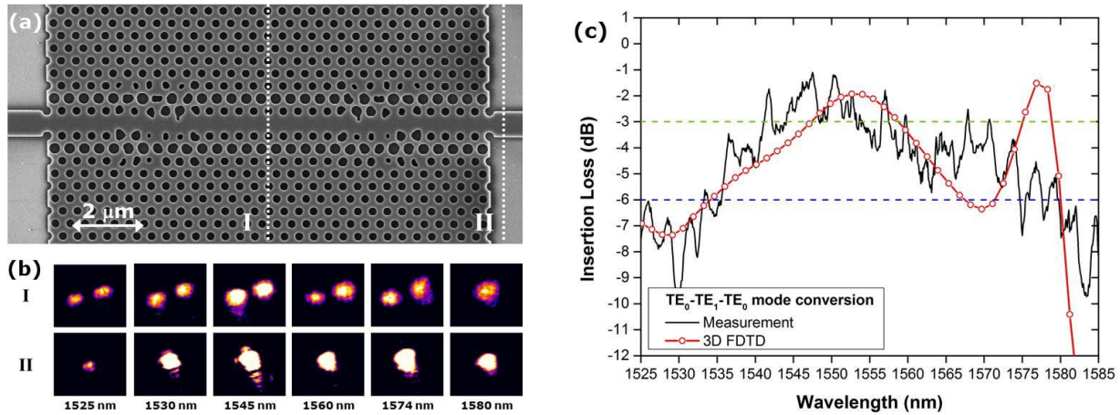
Fig. 2. (a) SEM image of the optimized TE_0 - TE_1 - TE_0 mode converter fabricated for characterization purpose in SOI material. (b) Mode profiles recorded for the TE_0 - TE_1 (I) and TE_0 - TE_1 - TE_0 (II) mode converters at given wavelengths. (c) Measured (black) and 3D FDTD calculated (red) insertion loss for the device.
