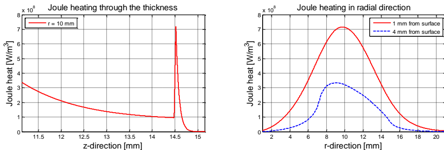
Fig.5. Joule heat distribution in different positions: Left: in the z -direction above the inductor (here, a high peak is observed in the magnetic layer). Right: in the radial direction at different distances from the mold cavity surface.
