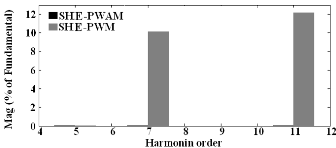
Fig. 11. 5th, 7th and 11th harmonics magnitude in both cases.
