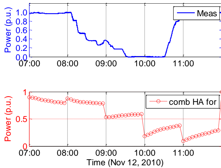
Figure 18. Measured vs intra-day forecasted power, November 12, 2010
