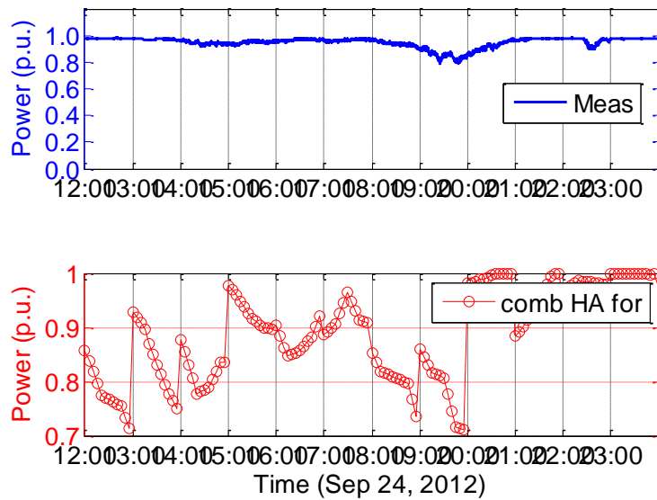
Figure 22. Measured vs intra-day forecasted power, September 24, 2012
