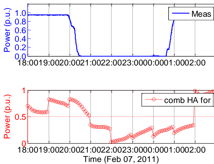
Figure 20. Measured vs intra-day forecasted power, February 7-8, 2011
