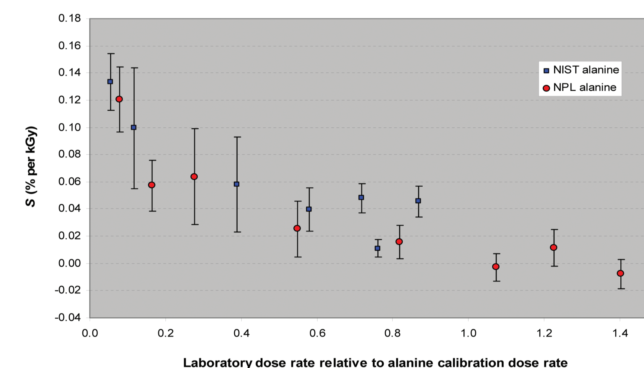
Figure 4. The slope S of the laboratory results R_{NIST} and R_{NPL} as a function of irradiation dose, plotted with respect to the laboratory dose rate relative to the alanine calibration dose rate. The uncertainty bars represent the standard uncertainty of S resulting from the linear regression. The results of the NIST irradiations of the NPL alanine at two dose rates are shown as separate points.
