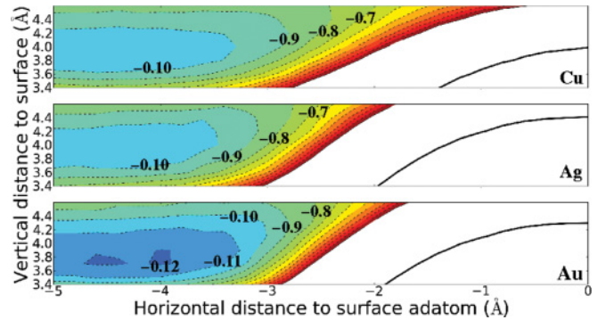
FIG. 5. (Color online) PES's for an Ar atom physisorbed on Cu, Ag, and Au(111) surfaces with an adatom of the same kind in the origin. The adsorption energy varies weakly between metals, Ar adsorption being slightly stronger on Au than on Ag, consistent with the lower polarizability of Ag. 34,35 The PES's also show the Ar preference for terrace away from the adatom. Black equipotential curve in white area, representing a 1 eV repulsion, calculated with revPBE, illustrates the strong repulsion at small separations and the approximate correlation of these curves with the coupling matrix element V_{ad} . 6 So, polarizability determines the strength of physisorptive attraction around the physisorption minima, while V_{ad} gives trend for the Pauli repulsion near the substrate.
