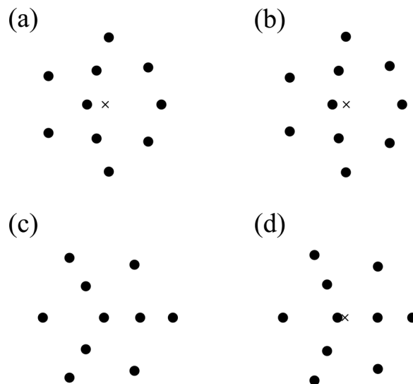
FIG. 2. Two examples, (a), (b) and (c), (d), of pairs of close relative equilibria for ten vortices.
