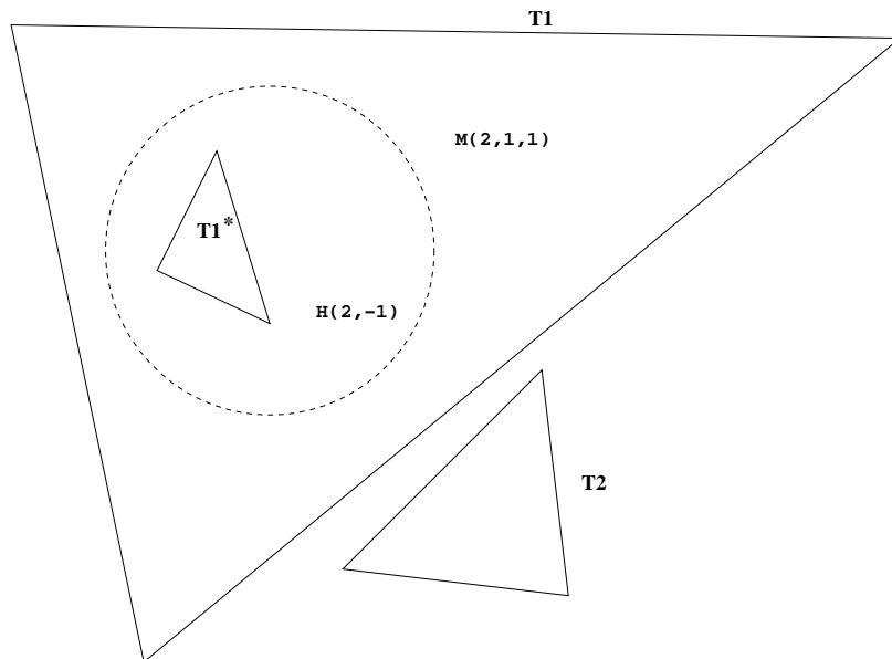
Figure 2.3: Projective model of \mathbb{H}(2, -1) and the upper hemisphere of \mathbb{M}(2, 1, 1) . The triangle \mathbf{T1} encloses the hyperbolic space and has a corresponding dual triangle \mathbf{T1}^* \subset \mathbb{H}(2, -1) , while the triangle \mathbf{T2} is not dual to a hyperbolic triangle.
