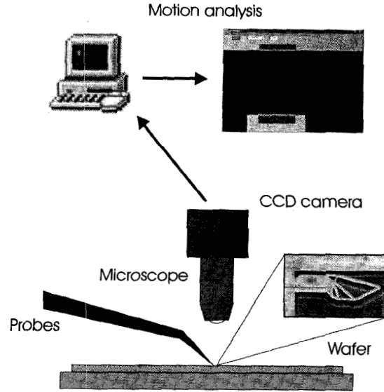
Figure 7. Experimental set-up. Images of the actuator work point, are acquired by a CCD camera and a framegrabber. Work point motion is determined by image analysis.
