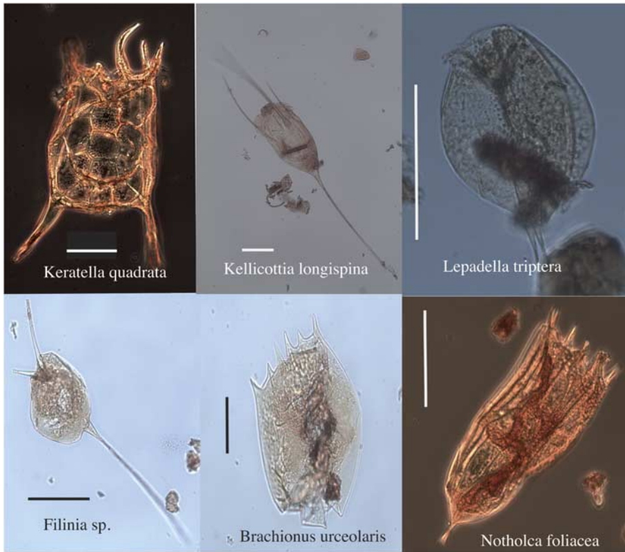
Fig. 1. Rotifers previously never recorded on the Antarctic continent, including: Filinia sp. (length without seta: 130 \mu\text{m} ); Kellicottia longispina (Kellicott) (length without spines: 170 \mu\text{m} ); Notholca foliacea (Ehrenberg) (length without spines: 135 \mu\text{m} ); Lepadella triptera (Ehrenberg) (length without spines: 75 \mu\text{m} ); Brachionus urceolaris Müller; (length without spines: 175 \mu\text{m} ); Keratella quadrata (Müller) (length without spines: 125 \mu\text{m} ). Scale bar in each part represents 50 \mu\text{m} . Picture: Jan-Erik Svensson.
