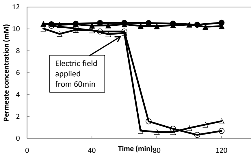
Figure 3.15 The permeate concentrations of Glu and Leu obtained without and with electric field applied at polarity +UF-, pH of feed solution stayed at 6.6 \pm 0.2 (▲) Leu at 0.5 bar and 60 A/m 2 (△) Glu at 0.5 bar and 60 A/m 2 (●) Leu at 0.3 bar and 60 A/m 2 (○) Glu at 0.3 bar and 40 A/m 2
