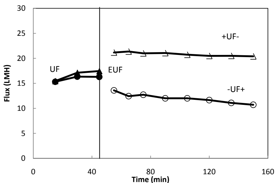
Figure 3.12 Flux change by applying electric field both at polarity +UF^- and -UF^+ during EMF of Glu-, ( \blacktriangle ) 0.28bar 0 A/m 2 ( \triangle ) 0.28bar 40 A/m 2 at polarity +UF^- ( \bullet ) 0.28bar 0 A/m 2 ( \circ ) 0.28bar 40 A/m 2 at polarity -UF^+
