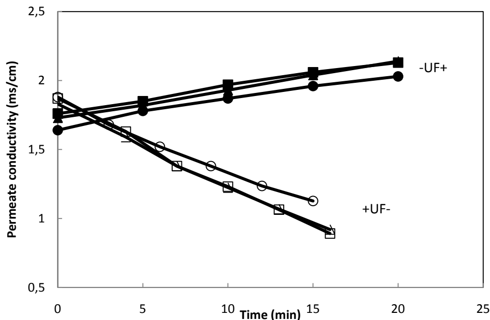
Figure 3.5 Permeate conductivity changes in the permeate reservoir at different TMP, polarities and at constant current density during EMF of NaCl ( 60\text{A/m}^2 and 20\text{A/m}^2 at polarity +UF- and -UF+ respectively) (■) 0.65bar (▲) 0.38bar (●) 1.16 bar (□) 0.47bar (△) 0.58bar (○) 0.97bar
