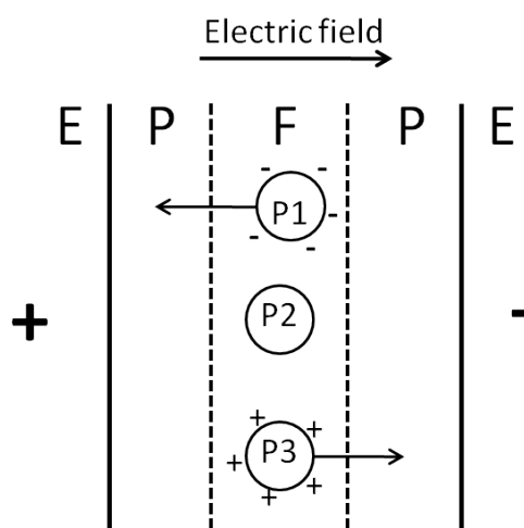
Figure 6.2 Demonstration of multicompartement for trinary mixture protein separation
