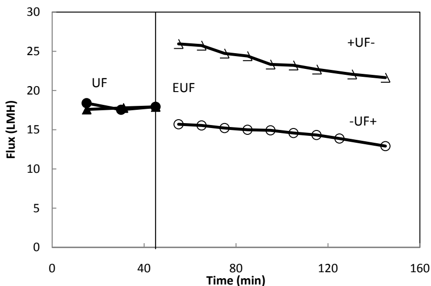
Figure 3.13 Flux change by applying electric field both at polarity +UF- and -UF+ during EMF of Lys+, ( \blacktriangle ) 0.28bar 0 A/m 2 ( \triangle ) 0.28bar 40 A/m 2 at polarity +UF- ( \bullet ) 0.28bar 0 A/m 2 ( \circ ) 0.28bar 40 A/m 2 at polarity -UF+
