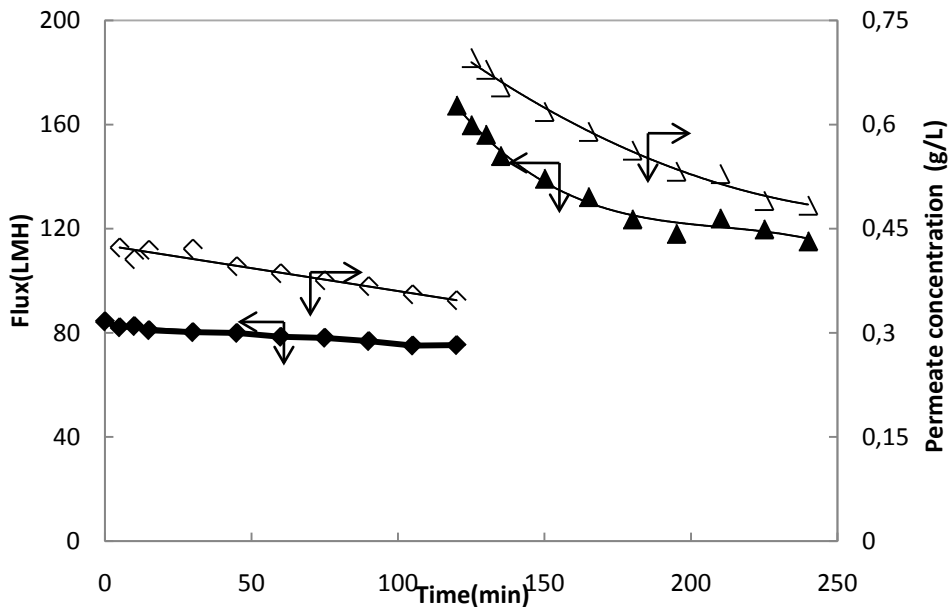
Figure 4.15 Permeate flux and concentration change as function of time at two constant TMPs during MF of BSA, (◆)Flux at 0.6bar(▲)Flux at 1.15bar(◇)BSA permeate concentration at 0.6bar(△) BSA permeate concentration at 1.15bar
