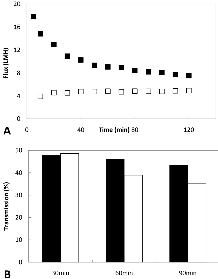
Figure 5.8(A) Permeate flux and (B) transmission comparison obtained from two different Batches of PLA during EMF of PLA, experiments were run with the same initial feed concentration 15g/L, feed pH 5, TMP 0.35bar and 1364V/m with polarity -MF+ (■) Batch A (□) Batch B
