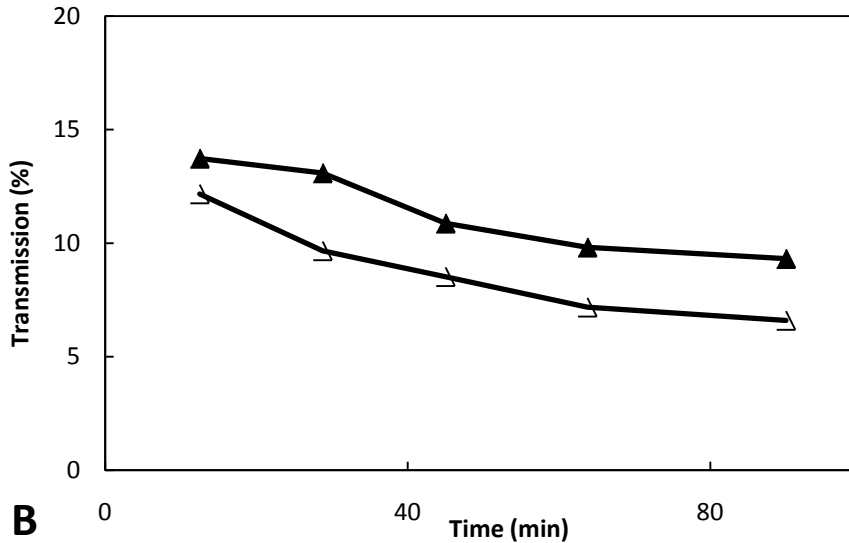
Figure 5.14 (A) Permeate flux and (B) PLA and LP transmissions obtained from the MF of PLA and LP, initial feed concentration 21.8g/L (PLA+LP) with 23.2% LP, pH 5, TMP 0.35bar (▲)PLA(△)LP
