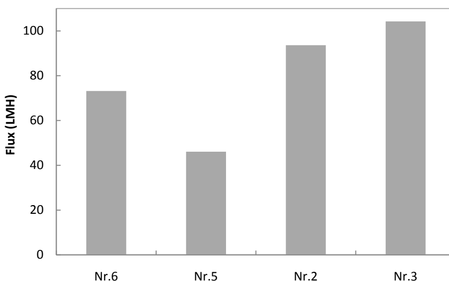
Figure 4.8 Comparison of the permeate flux obtained from different feed pH during UF of BSA (data obtained before the EUF operation); Exp. Nr.6 pH 3.8 \pm 0.3 , Nr5 pH 5.4 \pm 1 , Nr.2 pH 7.6 \pm 0.7 , Nr.3 pH 8.9 \pm 0.2
