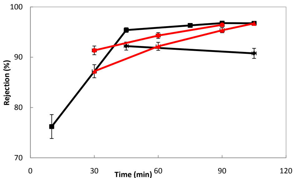
Figure 4.11 Comparison of the rejections obtained from difference feed pH during EUF of BSA at polarity -UF+ , ( \blacklozenge ) Nr.6 pH 3.8\pm 0.3 , ( \blacksquare ) Nr.5 pH 5.4\pm 1 ( \blacktriangle ) Nr.2 pH 7.6\pm 0.7 ( \bullet ) Nr.3 pH 8.9\pm 0.2
