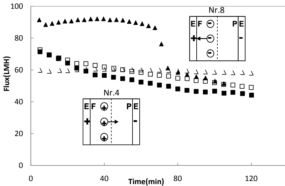
Figure 4.24 Comparison of the permeate flux obtained at different feed pH during MF and EMF of BSA at polarity+MF- of BSA (■)EMF Nr.4, pH 3.2±0.5(□) MF Nr.5,pH 3.8±0.3(▲)EMF Nr.8,pH 7±3.1 (Δ)MF Nr.7,pH 9.5±0.4 (details on experimental condition for Exp. Nr.5 and Nr.7 can be referred to Table 4.3)
