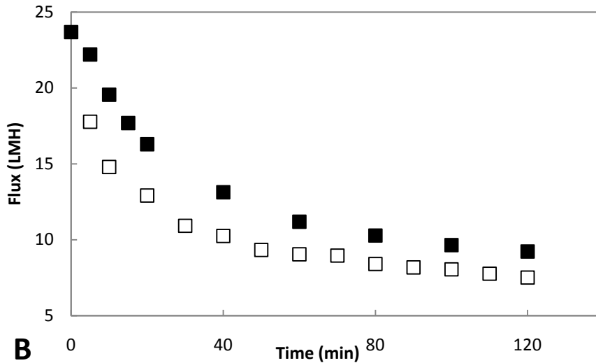
Figure 5.7 (A)Transmission of PLA and (B) permeate flux obtained from MF filtration with and without electric field, initial feed concentration 15g/L, pH 5, TMP at 0.35bar (■)MF (□)-MF+ at constant electric field strength 1364V/m
