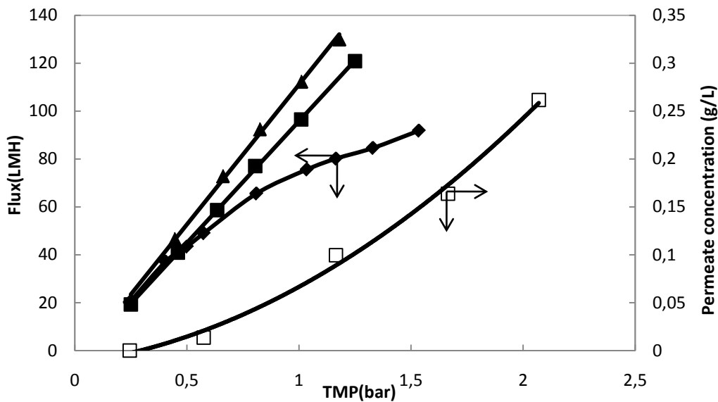
Figure 4.2 Permeation flux and permeate concentration of BSA as function of TMP from Exp. Nr.A during UF of BSA (refer to Table 4.1, UF filtration of BSA at pH around 7)(■)H 2 O flux after exp.(▲) H 2 O flux before exp. (◆)Permeate flux during exp.(□)BSA permeate concentration
