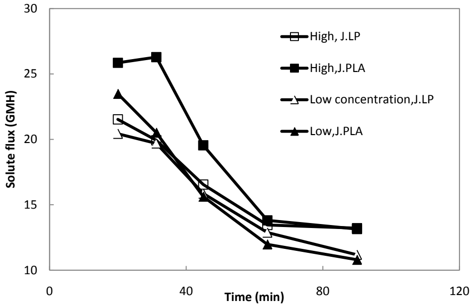
Figure 5.21 Effect of feed concentration on solute flux of PLA and LP during EMF operation (■)PLA, 19.1g/L (□)LP, 19.1g/L (▲)PLA, 10.2g/L (Δ)LP, 10.2g/L
