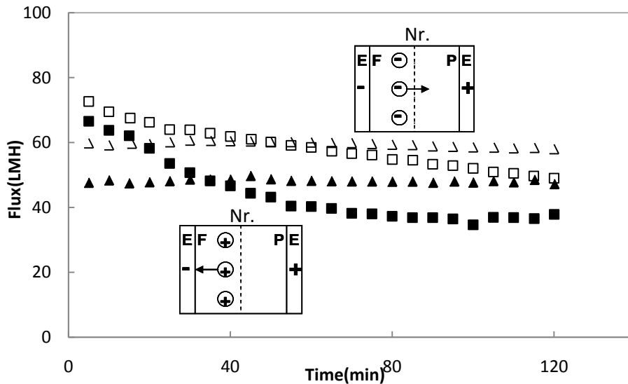
Figure 4.27 Comparison of the permeate flux obtained at different feed pHs during MF and EMF of BSA at polarity-MF+ (■)EMF Nr.3, pH 4.7±1.2 (□) MF Nr.5,pH 3.8±0.3(▲)EMF Nr.6,pH 9.5±0.4 (Δ)MF Nr.7,pH 9.5±0.4 (details on experimental condition for Exp. Nr.5 and Nr.7 can be referred to Table 4.3)
