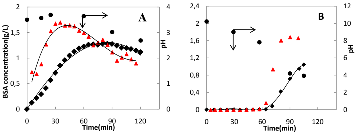
Figure 4.23 Comparison of the measured and calculated permeate BSA concentration obtained at different feed pHs during EMF of BSA at polarity +MF- (A) Exp. Nr.4 acidic pH 3.19±0.5 (B) Exp. Nr.8 basic pH 7±3.1 (details refer to Table 4.5) (◆)Cp.bulk measured(▲)Cp.calculated(●)Feed solution pH
