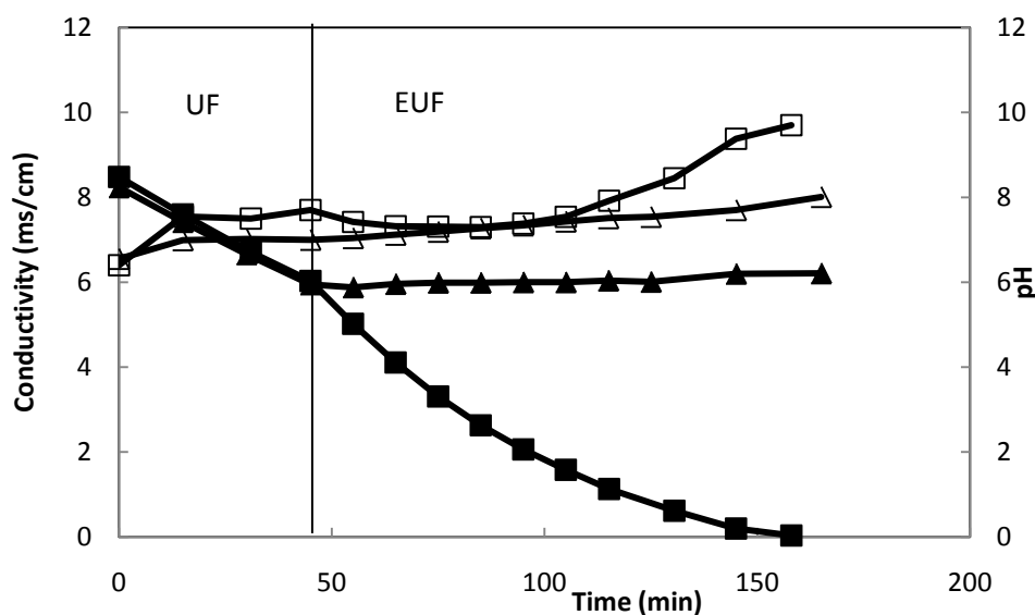
Figure 3.10 Conductivity and pH changes in permeate compartment during EMF of Lys, (■) Conductivity +UF- (□) pH +UF- (▲) Conductivity -UF+ (△) pH -UF+
