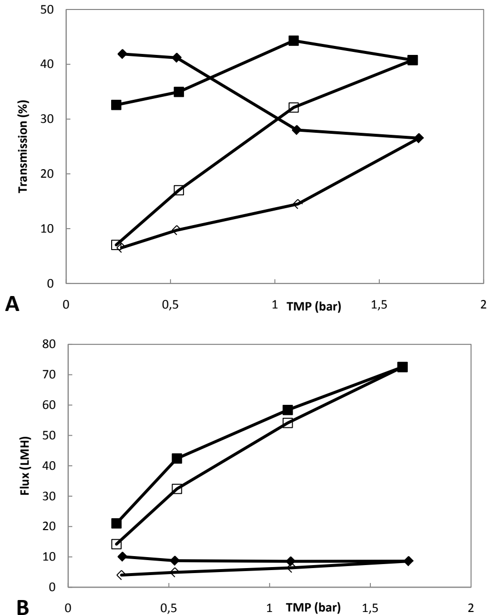
Figure 5.10 (A) Transmissions and (B) permeate flux during the step-up and step-down MF experiments, feed concentration 2g/L LP (■) pH 7.2, step-up (□)pH 7.2, step-down (◆)pH 4.7, step-up(◇)pH 4.7, step-down
