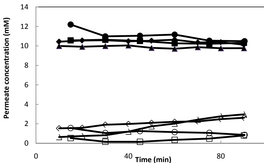
Figure 3.16 The concentration change of Leu and Glu in permeate compartment at different combinations of current and TMP at polarity +UF- (■)Leu at 0.6 \text{ A} 0.3 \text{ bar} (□)Glu at 0.6 \text{ A} 0.3 \text{ bar} (▲)Leu at 0.6 \text{ A} 0.5 \text{ bar} (△)Glu at 0.6 \text{ A} 0.5 \text{ bar} (●)Leu at 0.4 \text{ A} 0.3 \text{ bar} (○) Glu at 0.4 \text{ A} 0.3 \text{ bar} (◆)Leu at 0.4 \text{ A} 0.5 \text{ bar} (◇)Glu at 0.4 \text{ A} 0.5 \text{ bar}
