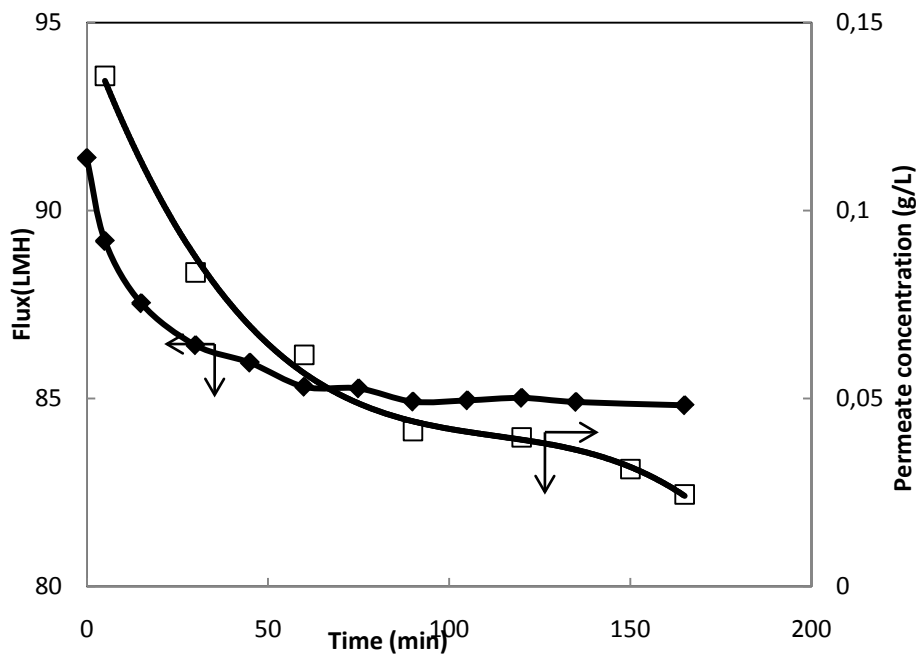
Figure 4.3 Permeate flux and permeate concentration of BSA at TMP 1.37bar from Exp Nr.B during UF of BSA (◆)Permeate flux (□)BSA permeate concentration
