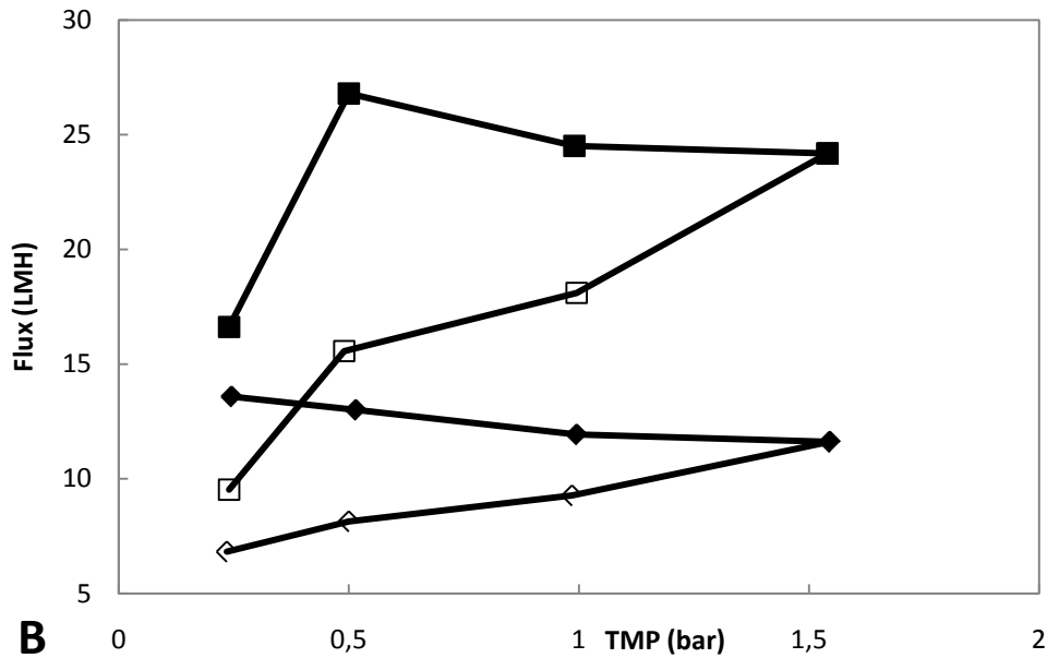
Figure 5.5 (A) The transmission of PLA and (B) permeate flux at 25min of each TMP obtained during MF of 15g/L PLA (■) pH 7.7, step-up (□) pH 7.7, step-down (◆) pH 4.7, step-up (◇) pH 4.7, step-down
