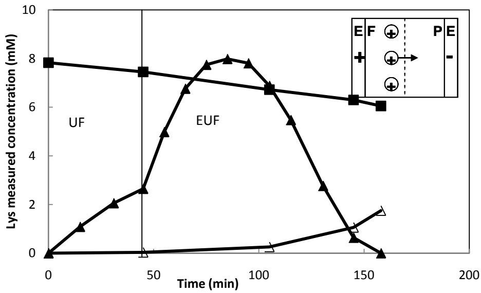
Figure 3.8 Lys concentration changes measured from the permeate and electrolyte compartment with and without the application of electric field at polarity +UF- at constant TMP 0.28 bar, feed pH at 7.2 \pm 0.2 (■) feed (▲) permeate(△) electrolyte
