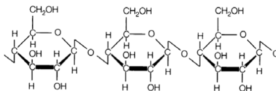
Figure 2.2 Structure of cellulose unit
