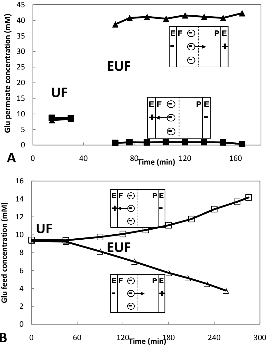
Figure 3.6 (A)Permeate concentration and (B)feed concentration of Glu with and without the application of electric field at different polarity, feed pH at 7\pm 0.5 during EMF of Glu (■) C_p 0.28bar 0/40 A/m 2 +UF- (▲) C_p 0.28bar 0/40 A/m 2 -UF+(□) C_f 0.28bar 0/40 A/m 2 +UF- (△) C_f 0.28bar 0/40 A/m 2 -UF+
