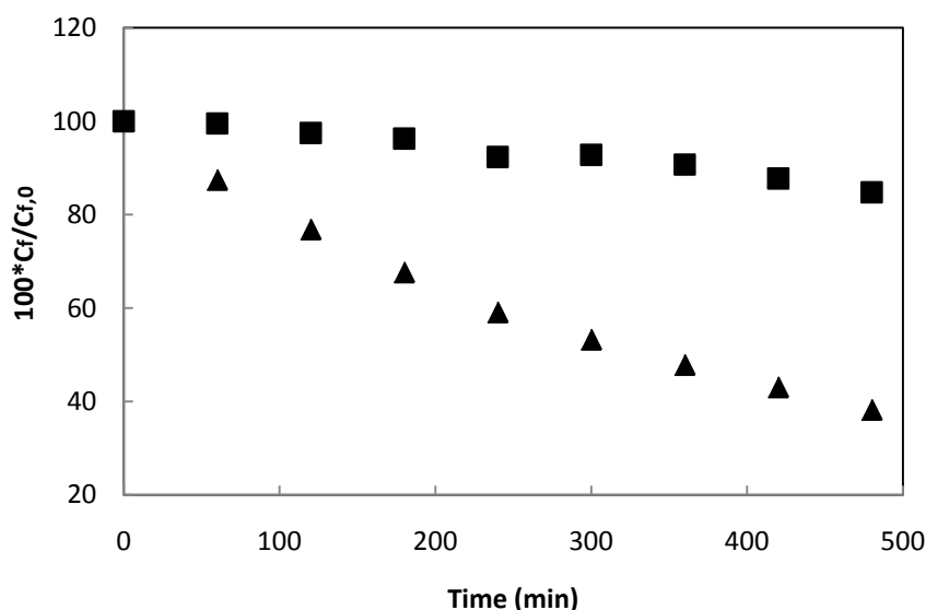
Figure 3.17 Changes of concentration ratio relative to the original feed concentrations of Leu and Glu during electrodiafiltration at polarity +UF-, current density 40 \text{ A/m}^2 , TMP 0.5 bar; 1.2L addition of water during the diafiltration of 1.1 L feed solution. Initial feed solution consisted of
