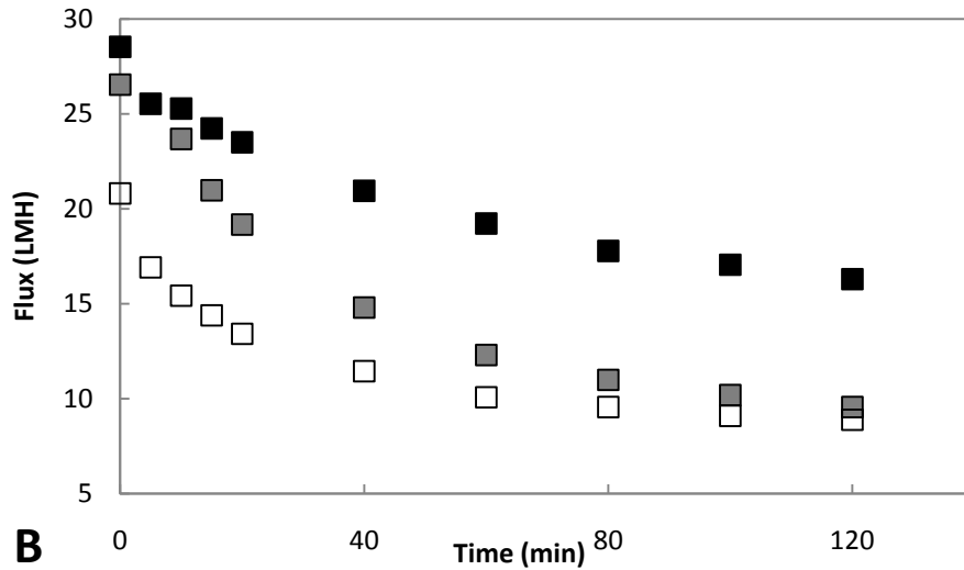
Figure 5.6 (A) Transmission of PLA and (B) permeate flux obtained at different solution pH during 2 hours' MF of 15g/L PLA at constant TMP 0.35bar (■)pH 7.7 (■)pH 5.4 (□)pH 4.7
