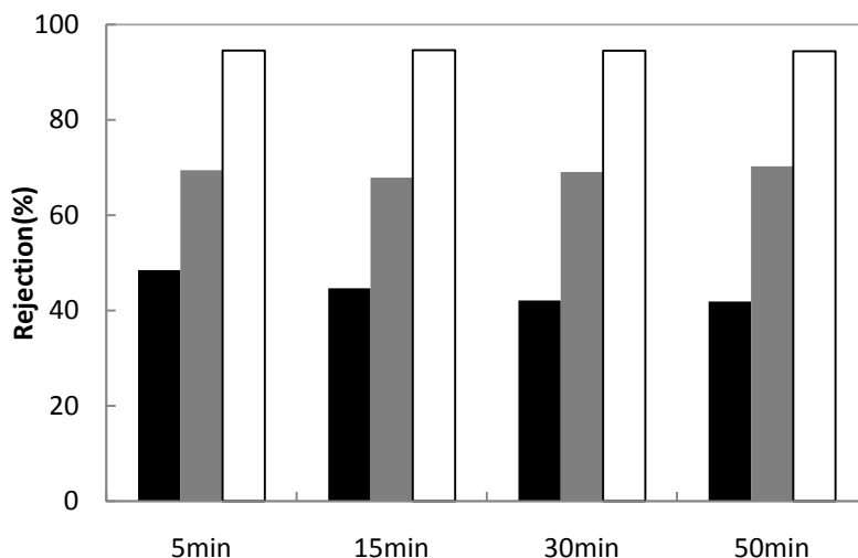
Figure 4.21 Comparison of rejections obtained at different feed pHs, constant TMP 0.6 bar during MF of BSA operated without permeate circulation (■) Exp.A, pH 3.6±0.9 (■) Exp.B, pH 6.8±0.3 (□) Exp.C, pH 9.8±0.2
