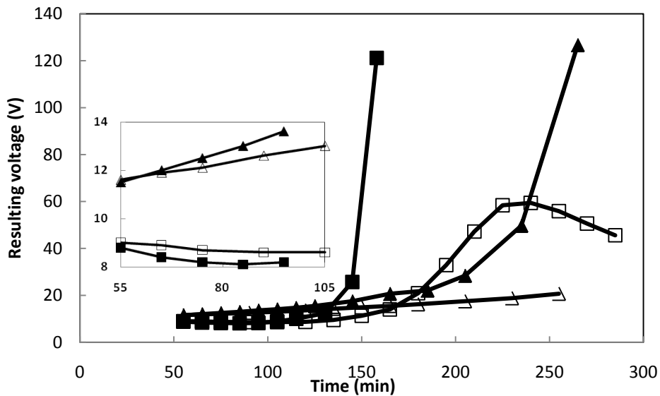
Figure 3.11 Variations of the resulting voltage in different operation conditions during EMF of Glu and Lys at current density 40\text{A/m}^2 , ( \blacksquare ) +UF-, \text{Lys}^+(\blacktriangle) -UF+, \text{Lys}^+(\triangle) -UF+, \text{Glu}^-(\square) +UF-, \text{Glu}^-
