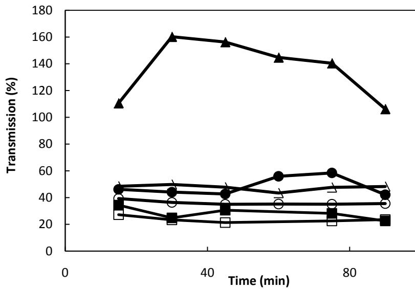
Figure 5.32 Comparison of the transmissions of PLA and LP obtained at different feed pHs during EMF of PLA and LP (■)Tr LP, pH 5(□)Tr PLA, pH 5 (●)Tr LP pH 5.25 (○) Tr PLA pH 5.25 (▲)Tr LP, pH 5.5(△) Tr PLA, pH 5.5
