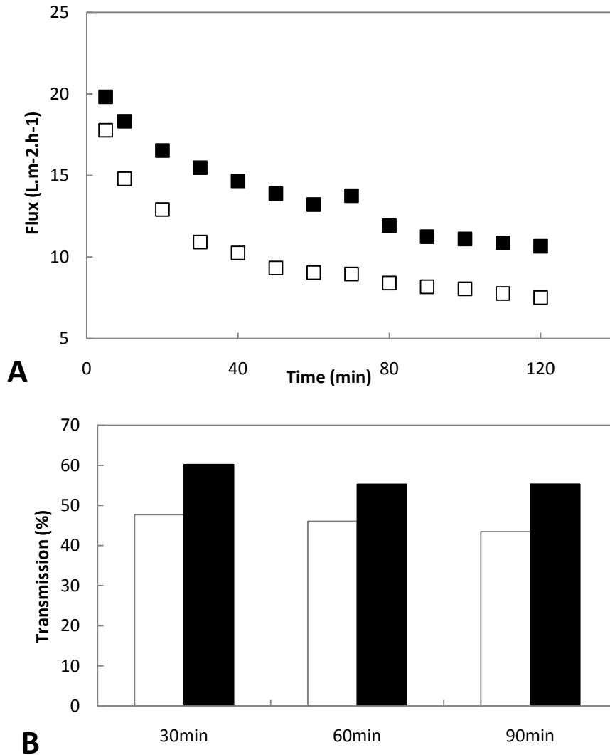
Figure 5.9 (A) Permeate flux and (B) transmission improvement by addition of 5mM Na 2 SO 4 , experiments were ran with the same initial feed concentration 15g/L (stock solution from Batch A), feed pH 5, TMP 0.35bar and 1364V/m with polarity –MF+(■) with addition of 5mM Na 2 SO 4 in the feed solution (□) without addition of Na 2 SO 4
