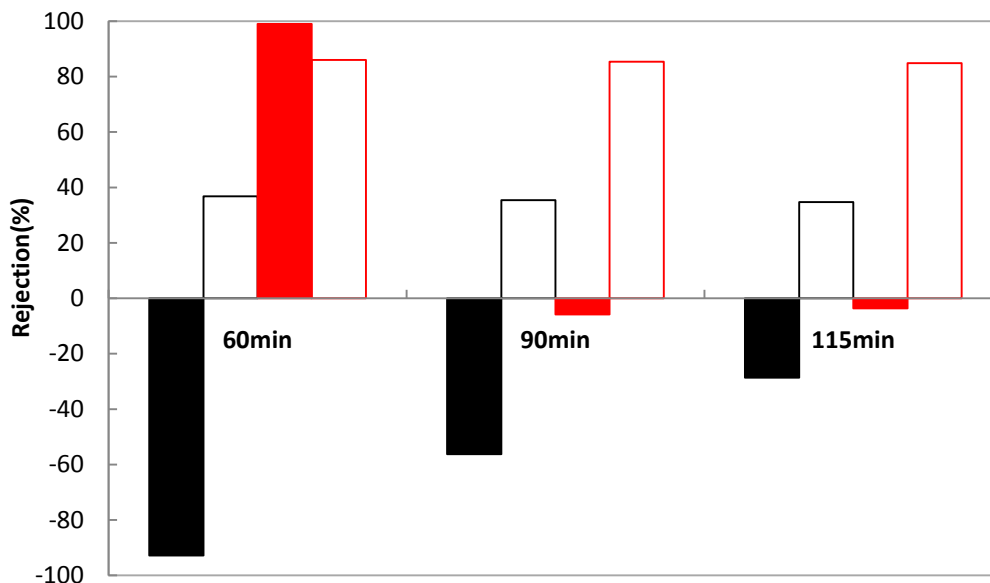
Figure 4.25 Comparison of BSA rejections obtained at different feed pH during MF and EMF of BSA at polarity+MF-, (■)EMF Nr.4, pH 3.2\pm 0.5 (□) MF Nr.5, pH 3.8\pm 0.3 (■)EMF Nr.8, pH 7\pm 3.1 (□)MF Nr.7, pH 9.5\pm 0.4 (details on experimental condition for Exp. Nr.5 and Nr.7 can be referred to Table 4.3)
