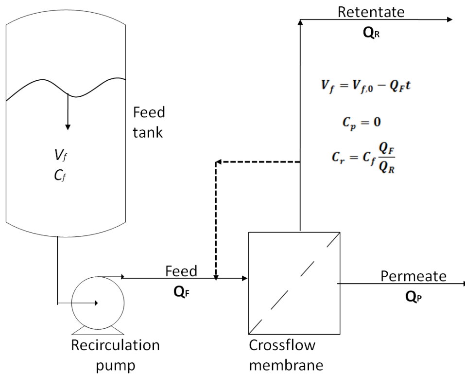
Figure 1.7 Diagrammatic of continuous concentration mode
