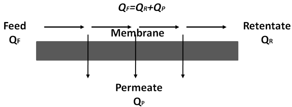
Figure 1.5 General scheme of crossflow membrane filtration
