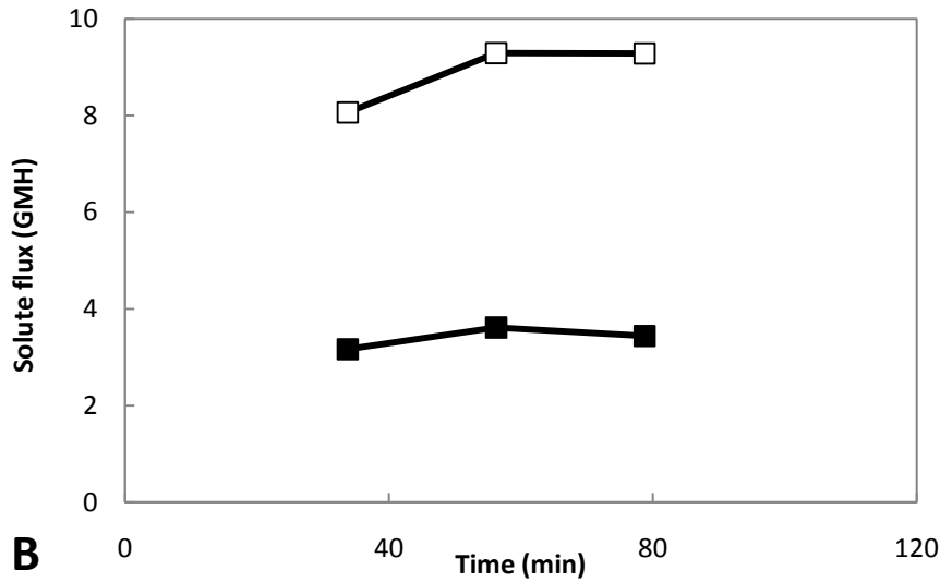
Figure 5.29 (A) Permeate flux and (B) solute flux of the two enzymes during EMF (■)LP (□)PLA
