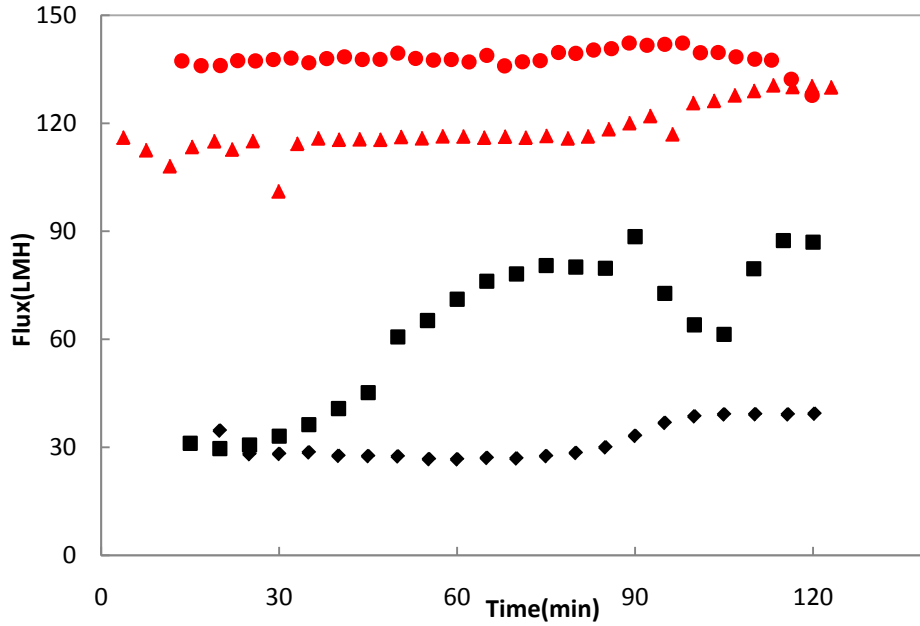
Figure 4.5 Comparison of the permeate flux changes obtained at different feed pH during EUF of BSA at polarity +UF- (◆)Nr.8, pH 3.7\pm 0.2 (■)Nr.4, pH 5\pm 0.5 (▲)Nr.1,pH 7.2\pm 0.4 (●)Nr.7,pH 9.7\pm 0.2
