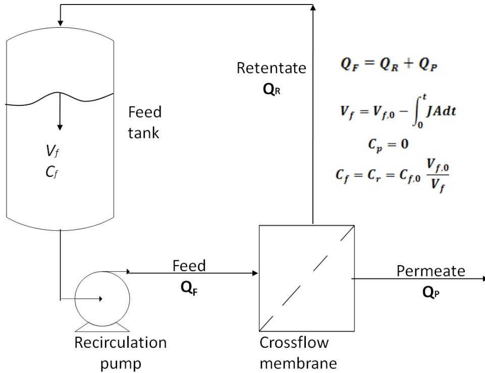
Figure 1.6 Diagrammatic of batch concentration mode
