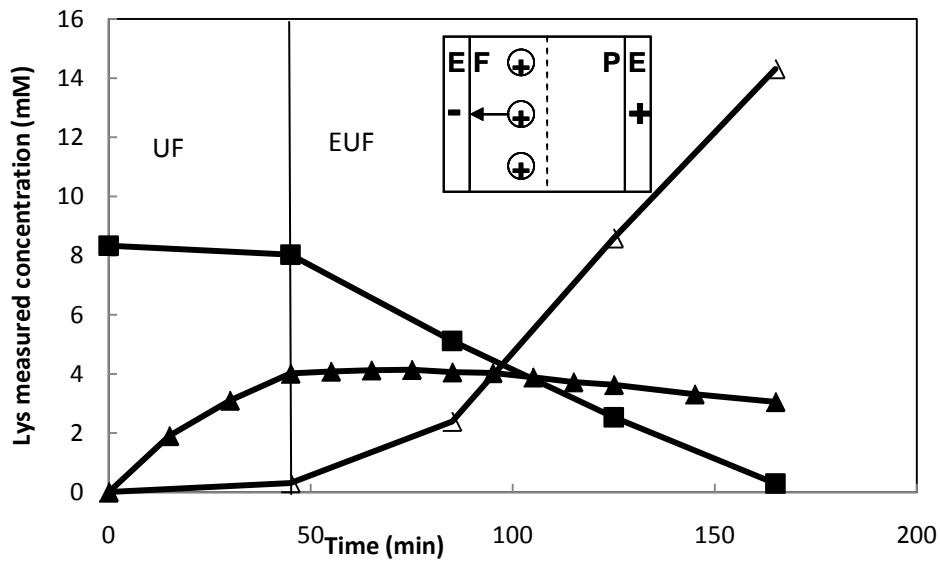
Figure 3.9 Lys concentration changes measured from permeate, feed and electrolyte compartments with and without the application of electric field at polarity –UF+ at constant TMP 0.28bar, feed pH at 7-9.5(■)feed(▲)permeate(△)electrolyte
