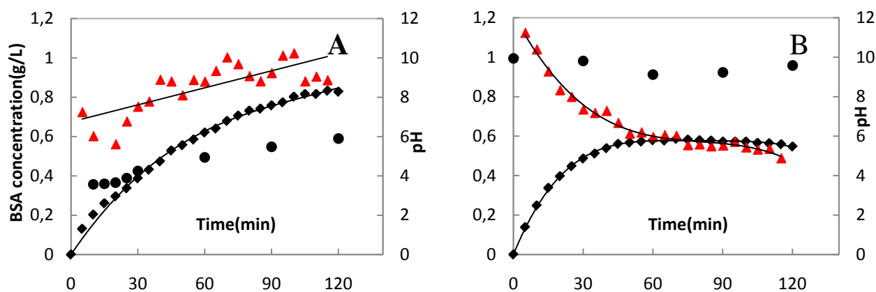
Figure 4.26 Comparison of the measured and calculated permeate BSA concentration obtained at different feed pHs during EMF filtration of BSA at polarity -MF+ , (A) Exp. Nr.3 acidic pH 4.7 \pm 1.2 (B) Exp.Nr.6 basic pH 9.5 \pm 0.4 (details refer to Table 4.5) ( \blacklozenge )Cp.bulk measured( \blacktriangle )Cp calculated( \bullet )Feed solution pH
