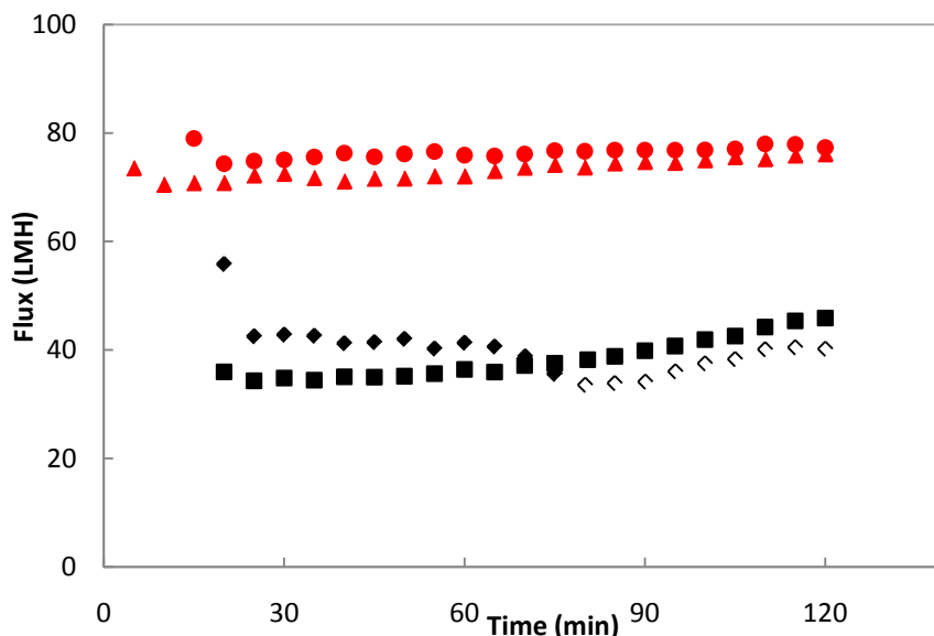
Figure 4.9 Comparison of the permeate flux changes obtained from different feed pH during EUF of BSA at polarity -UF+ (◆) Nr.6 pH 3.8\pm 0.3 , 909V/m (◇) Nr.6 pH 3.8\pm 0.3 , 1818V/m (■) Nr.5 pH 5.4\pm 1 (▲) Nr.2 pH 7.6\pm 0.7 (●) Nr.3 pH 8.9\pm 0.2
