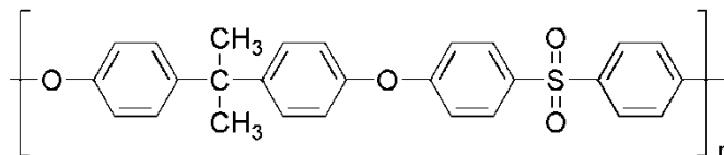
Figure 2.1 Structure of polysulfone unit
