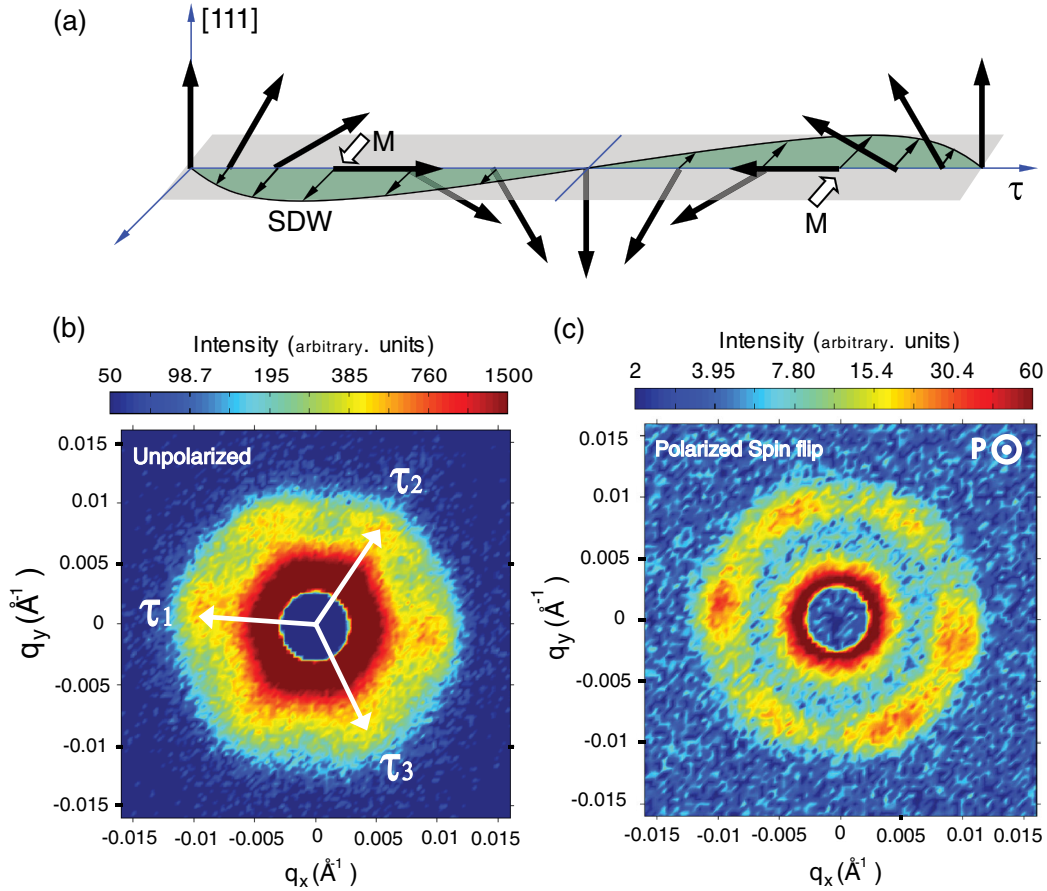
FIG. 1 (color online). (a) The SDW (thin arrows normal to both [111] and \tau ) produced by the tilt of the Fe spins out of the plane of the magnetic cycloid (thick arrows in the plane defined by [111] and \tau ). The amplitude of the SDW is exaggerated. Only a few representative spins are shown. Open arrows show local magnetization due to the SDW. (b) and (c): Images of the diffraction pattern in the (111) scattering plane with (b) unpolarized neutrons, (c) neutrons polarized with \mathbf{P} \parallel beam that scatter with spin flip. The images were prepared by summing several detector measurements over a range of rocking angles \beta (see text), allowing all Bragg reflections from the long-wavelength modulation to be presented in a single image. A beam stop blocks the direct beam in the center of each image.
