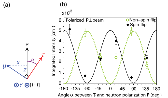
FIG. 3 (color online). Data for neutrons polarized with \mathbf{P} \perp beam, in the vertical direction on the detector. (a) Schematic in detector plane illustrating the relationship between \mathbf{P} , \tau , and the components (X, Y, Z) of the vector \mathbf{T} associated with the magnetic modulation. (b) Dependence on the angle \alpha between \tau and \mathbf{P} of the polarized neutron intensities for all Bragg spots \pm\tau_i , each integrated over its rocking curve and normalized by its relative domain population. Both the SF and NSF channels are shown. The lines are fits described in the text.
