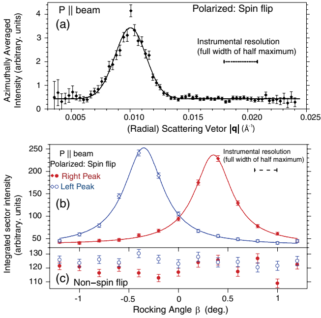
FIG. 2 (color online). Details of the \pm\tau_1 diffraction spots [left and right spots in Figs. 1(b) and 1(c)], using neutrons polarized with \mathbf{P} \parallel beam. Corrections for the polarizing efficiency of the instrument have been included. (a) |\mathbf{q}| dependence of azimuthally averaged intensity through both left and right spots at the peaks of their rocking curves. The solid line depicts a Gaussian fit. (b) and (c): Rocking curves for both left and right spots in the SF (b) and NSF (c) channels. The solid lines are Lorentzian fits. The dashed and dotted bars in these figures illustrate aspects of the experimental resolution discussed in the text. 55^\circ -wide sectors on the detector were used to pick out the \pm\tau_1 spots; similar results may be obtained with smaller sectors and/or by examining another pair of diffraction spots \pm\tau_2 , \pm\tau_3 .
