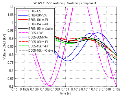
Fig. 3 Phase L3 to phase L1 voltage at the WTs DC05 and EF06 converter terminals from 150ms to 152ms for different PSCAD models.
