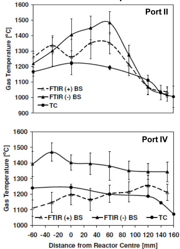
Figure 15 Temperature profiles measured by the FTIR-probe and the S-type thermocouple during coal fired experiments. NP = Normal purge flow, HP = High purge flow (2 x NP), BS = Beam stop, TC = Thermocouple.
