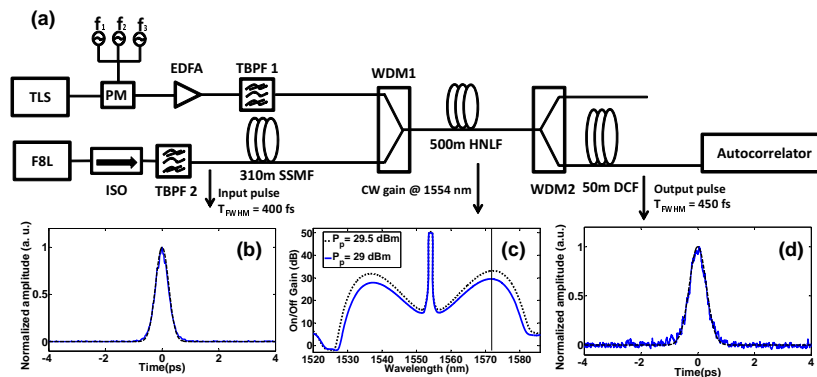
Fig. 1. (a) Experimental setup of the FOPCPA for the pulses dynamic characterization. (b) Autocorrelation trace of the 400 fs input pulse. (c) CW FOPA gain for two different pump levels (the vertical line indicates the signal central wavelength). (d) compressed output pulse autocorrelation measured with the pump signal switched off.
