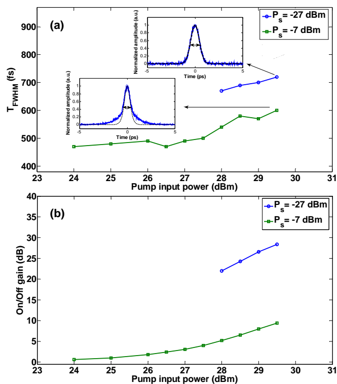
Fig. 2. (a) Pulwidth of the amplified signal as a function of pump power at the input of the HNLF in the saturated ( P_s = -7 dBm) and unsaturated ( P_s = -27 dBm) regimes. The insets show selected autocorrelation traces. (b) Corresponding measured on/off gain.
