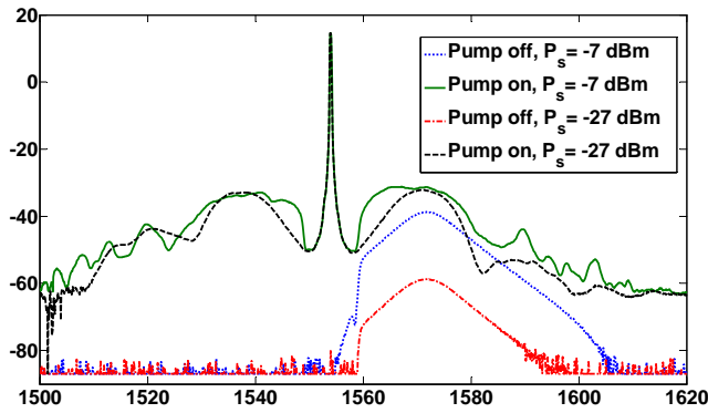
Fig. 3. Optical spectra measured at the output of the HNLF with the pump switched off and on ( P_p = 29 dBm) for P_s = -27 dBm and P_s = -7 dBm.
