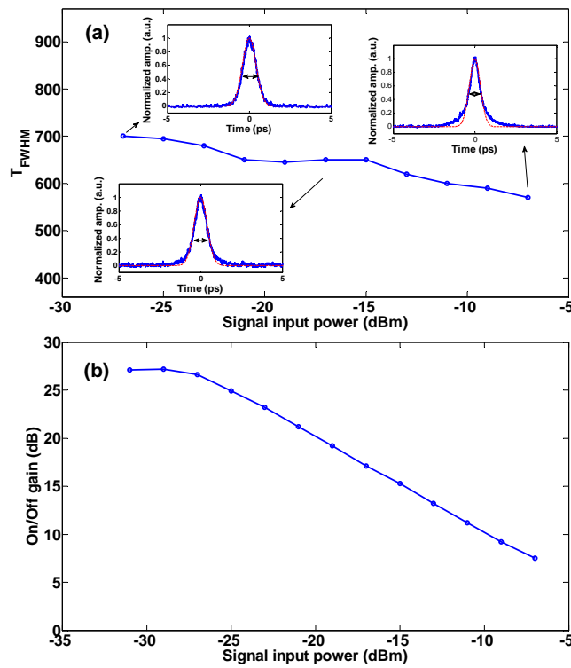
Fig. 4. (a) Pulsewidths of the amplified signal as a function of the signal input average power with a pump power of 29 dBm. The insets show selected autocorrelation traces. (b) Corresponding measured on/off gain.
