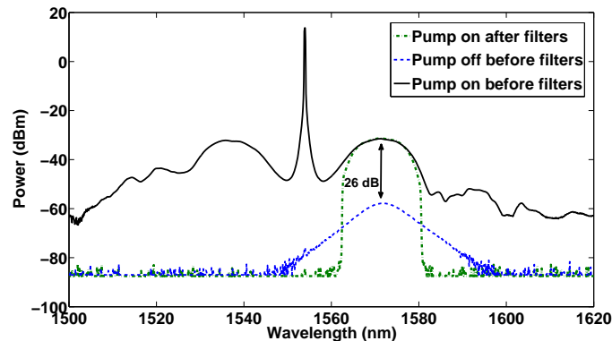
Fig. 7. Optical spectra measured at the output of the HNLF with the pump switched off (dashed blue line) and on (solid black line) with a pump power of 29 dBm.
