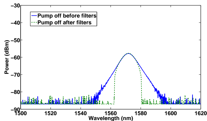
Fig. 6. Optical signal spectra measured at the output of the HNLF (solid line) and at the output of the filtering stage (dash-dot line) with the pump switched off.
