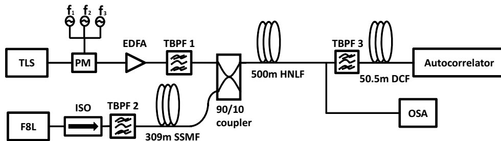
Fig. 5. Experimental setup of the FOPCPA for the amplification of the 400 fs pulses with a pump input power of 29 dBm and signal input average power of -27 dBm.
