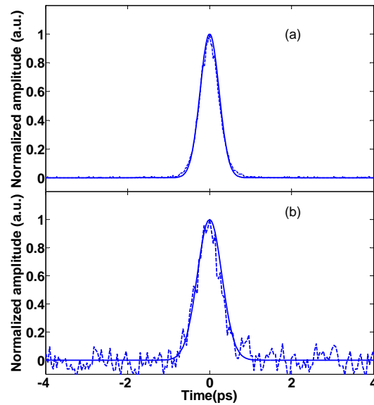
Fig. 8. Autocorrelation traces of the signal (a) at the input of the SSMF, corresponding to a pulsewidth of 400 fs and (b) at the output of the DCF, corresponding to a pulsewidth of 500 fs.
