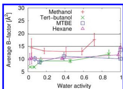
Figure 11. Average B-factor of CALB (omitting residues 1–20 and 308–317) vs water activity in methanol (+), tert -butyl alcohol (×), MTBE (□), and hexane (△). Standard error estimates were based on three replica simulations which were started from different initial velocities. Error bar limits for the average B-factor in pure water are marked by horizontal lines.
