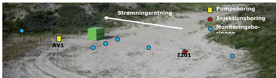
Figur 1 Boringsplacering
