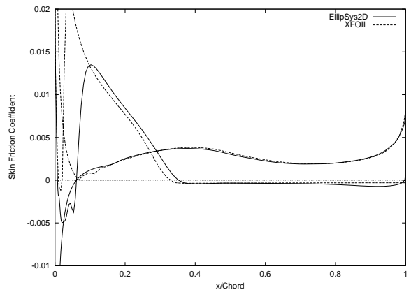
(f) \alpha = 20.33^\circ
