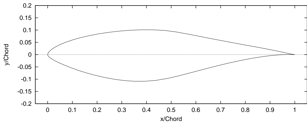
Figure 125. S809 Airfoil
