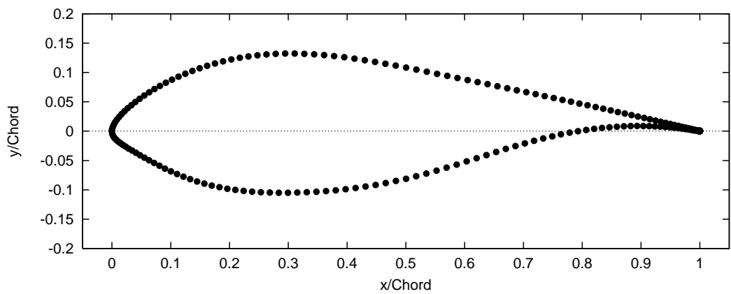
Figure 95. RISØ-A1-24 Airfoil
