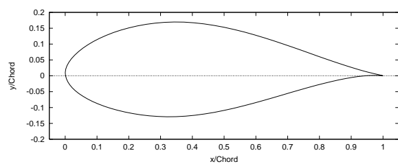
(a) NACA 63-430 Airfoil
