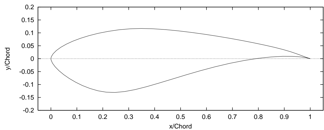
Figure 131. S814 Airfoil
