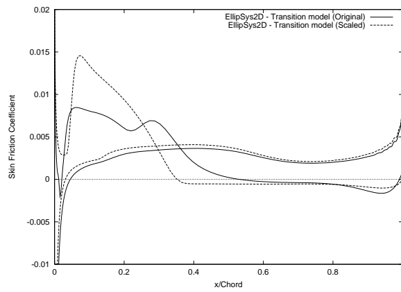
(f) Skin Friction Coefficient - \alpha = 15.11^\circ
