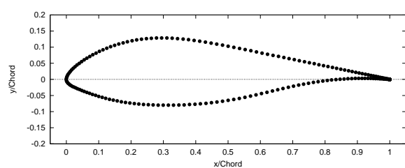
(c) RISO-A1-21 Airfoil
