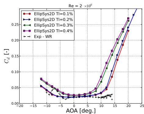
Figure 7: Lift and drag coefficients for the flat-back airfoil at Re=2 \times 10^6 computed with different inflow turbulence intensities.
