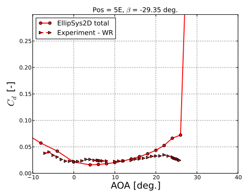
Figure 8: Lift and drag coefficients for the slatted airfoil with the slat in position 5E tested at Re=2 \times 10^6 . Note that the total lift is normalized with the main airfoil chord, while the lift coefficients for each element is normalized with their respective chord lengths.
