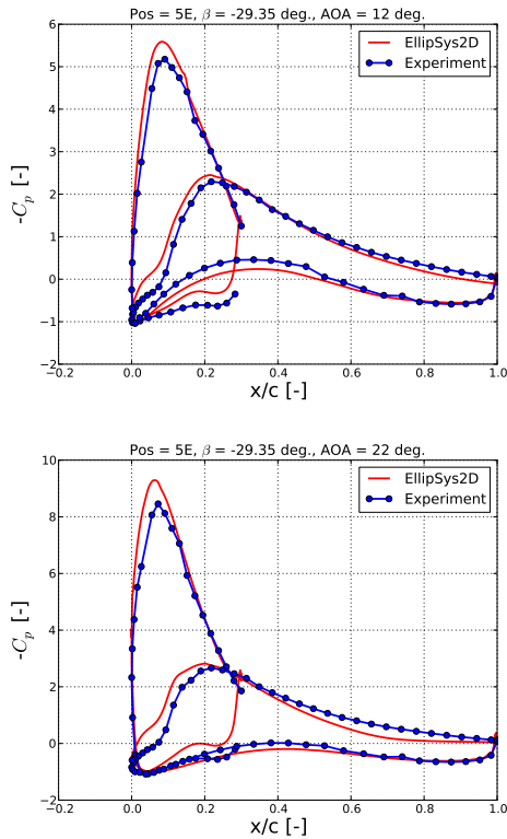
Figure 9: Pressure coefficients for the slatted airfoil with the slat in position 5E tested at Re=2 \times 10^6 . Note that the pressure distributions for both elements are plotted from x/c=0 although this is not their actual positions.
