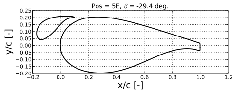
Figure 2: Optimized multiple element airfoil configuration .
