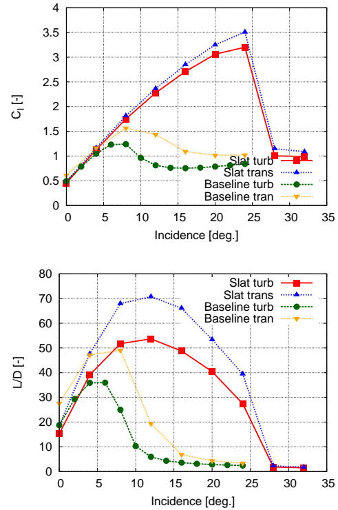
Figure 3: 2D lift coefficient and lift to drag ratio as function of incidence for fully turbulent and transitional boundary layers (TI=0.1%).
