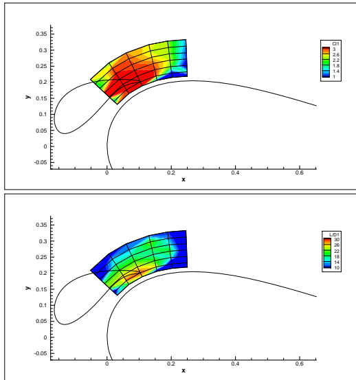
Figure 4: Parameter study of slat positioning showing contours of C_{l-max} and L/D at \alpha_{C_{lmax}} .
