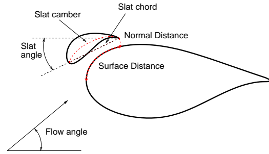
Figure 1: Geometrical parameters that the optimization code can adjust to meet the optimization targets.
