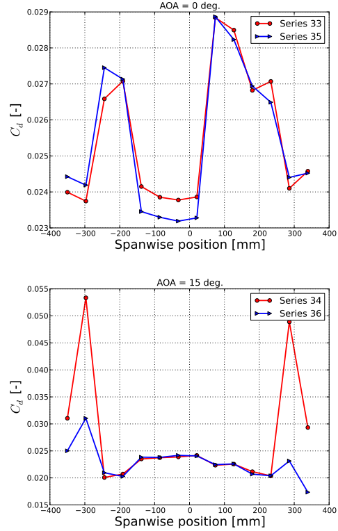
Figure 11: Drag coefficient as function of lateral measurement position for the multi-element airfoil with the slat in position 5E tested at Re=2 \times 10^6 . 0 mm is the center of the tunnel. The total tunnel width is 1400 mm.
