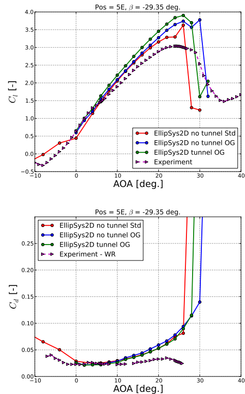
Figure 10: Lift and drag coefficients for the multi-element airfoil with the slat in position 5E tested at Re=2 \times 10^6 in a 2D tunnel configuration.
