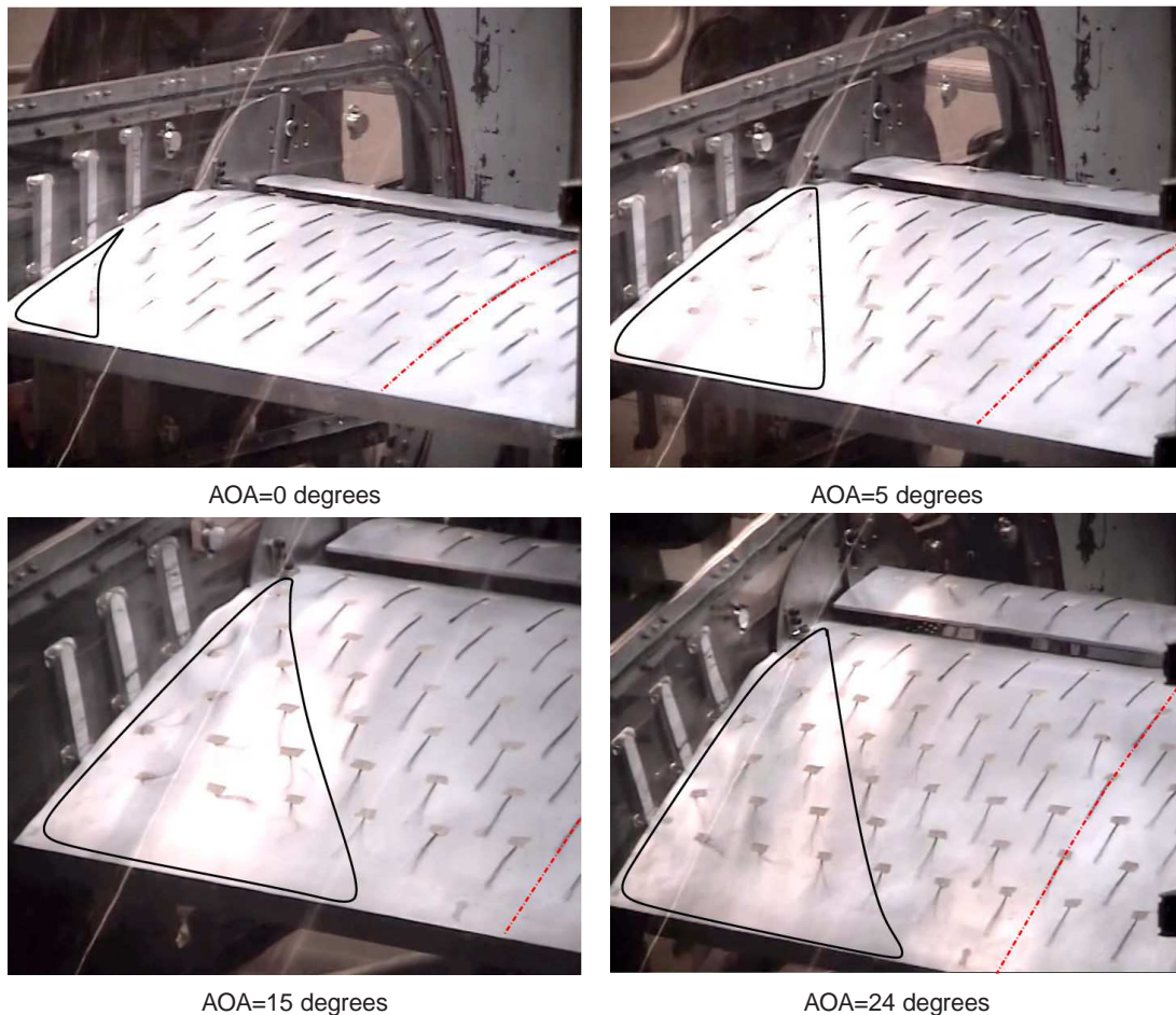
Figure 12: Wool tufts flow visualization of the slatted airfoil at various angles of attack.
