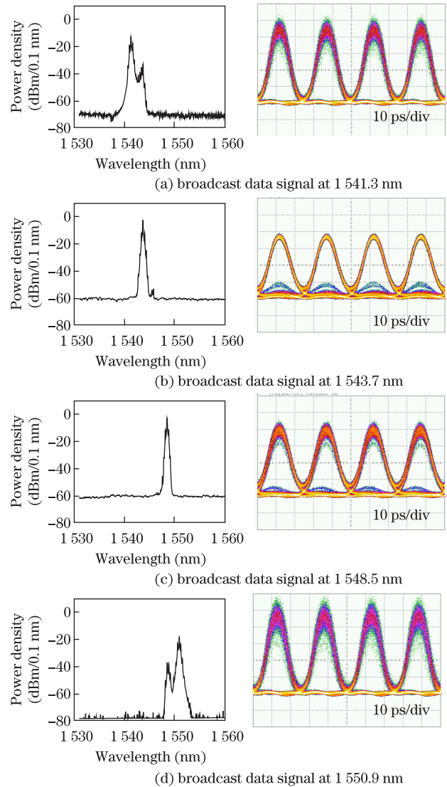
Fig. 3. (Color online) Optical spectra and eye diagrams of the broadcast data signals after filtering the subsystem at (a) 1541.3 , (b) 1543.7 , (c) 1548.5 , and (d) 1550.9\ \text{nm} .
