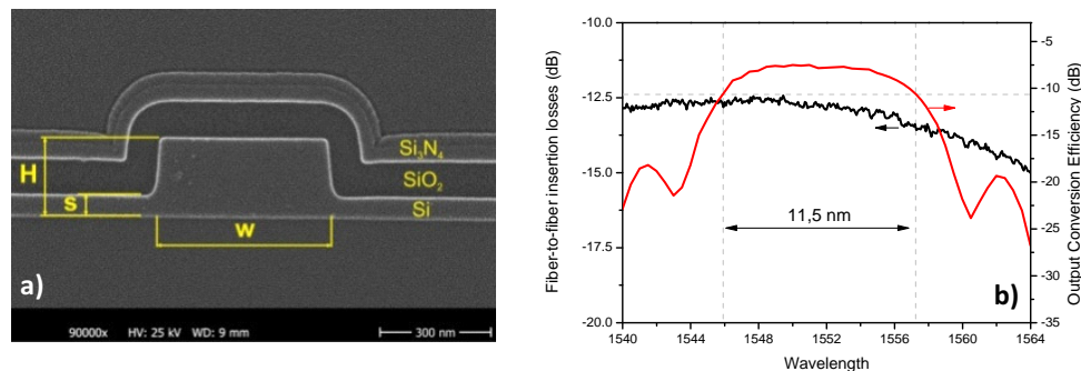
Fig. 1. (a) SEM picture of the cross-section of a silicon nano-rib waveguide: width W=500 \text{ nm} , height H=210 \text{ nm} and slab height s=50 \text{ nm} . (b) Fiber-to-fiber insertion losses and conversion efficiency bandwidth (pump at 1552 \text{ nm} ) as a function of the signal wavelength.
