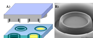
Figure 2. A) Graphics illustrating the hot embossing process after the stamp is released from the polymer film. B) SEM image of one PLLA microcontainer.
