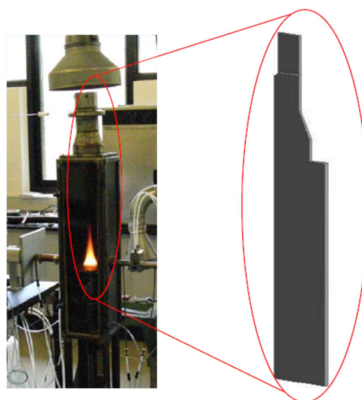
Figure 1: Experimental flame chamber with illustration of computational model domain.
