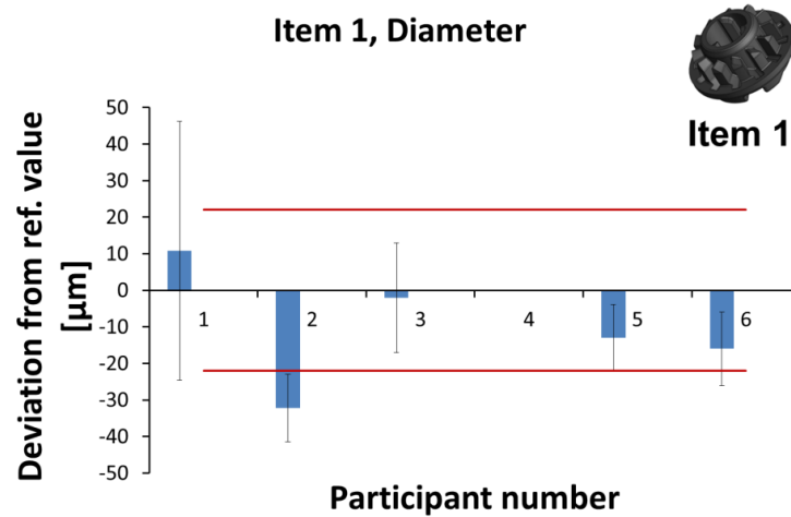
Figure 25: Deviation chart comparing the results obtained from all the participants except from participant no. 4 for Item 1 in the case of outer diameter. The red lines indicate the maximum reference uncertainty.
