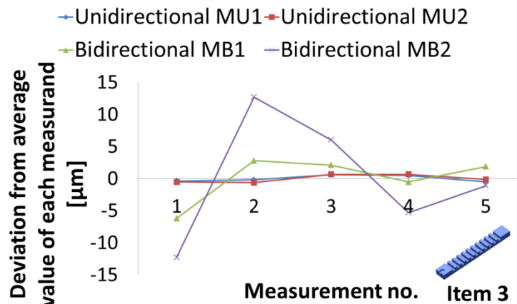
Figure 19: Variation of five reversal measurements. Note that for all the measurements, Item 3 was not moved (repeatability).
