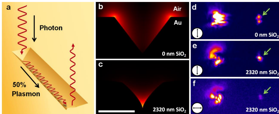
Fig. 2. (a) Illustration of the in- and out-coupling of light in the V-groove devices. (b)-(c) 2D FEM calculations of the electric field for different V-groove cross-sections. Scale bar is 2 \mu\text{m} . (d)-(f) Experimentally observed radiation from V-groove samples. Circular inset denotes the incident electric field polarization. \text{SiO}_2 layer modification alters the propagating mode distribution. The polarization dependence indicates a CPP mode.
