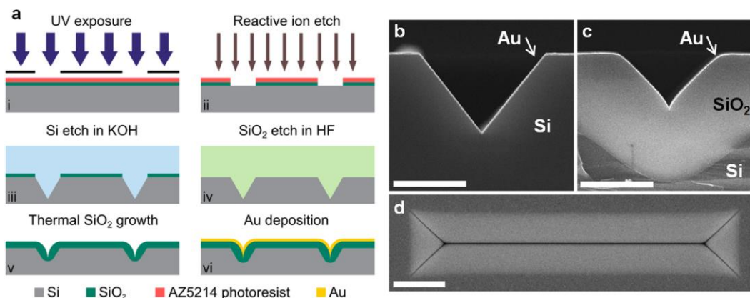
Fig. 1. (a) Fabrication procedure for Au V-grooves and coupling mirrors involving UV-lithography. (b)-(d) SEM images of resulting V-grooves, scale bars are 2 \mu\text{m} . (b) V-groove without thermal oxidation. (c) V-groove with a 2320 nm SiO 2 layer. (d) Top view of (c).
