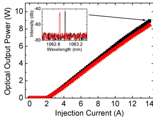
Fig. 2. Power current characteristics for both DBR-tapered diode lasers (Squares: transmitted laser, Triangles: diffracted laser). Both lasers are operated at 300 mA to the ridge waveguides and operating temperatures set to 20 °C. The inset shows the corresponding spectra emitted at 14 A to the tapered amplifiers.
