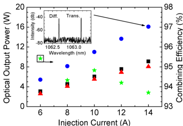
Fig. 3. Optical output power of the individual DBR-tapered diode lasers and the combined beam (Squares: transmitted laser, Triangles: diffracted laser, Circles: combined beam). The star symbols represent the corresponding combining efficiency. The inset shows the corresponding spectra emitted at maximum currents.
