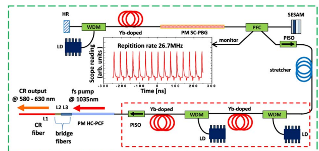
Fig. 1. (Color online) Layout of the all-fiber Cherenkov source. HR, high-reflectivity pigtailed mirror; WDM, 980/1030 wavelength division multiplexer; LD, single-mode pumping diode at 974 nm; PM SC-PBG, polarization-maintaining all-solid photonic bandgap fiber; SESAM, semiconductor saturable absorber mirror; PISO, polarization-maintaining isolator; PFC, 80/20 polarization filter coupler; HC-PCF, laser pulse compressor hollow-core PCF; CR fiber, highly nonlinear fiber for CR generation. (Inset) Oscilloscope reading of the mode-locked pulse train.
