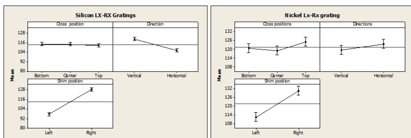
Figure 3: Main effect plot for fabricated geometries. Error bars indicate experimental expanded uncertainty ( U_{exp_{Si}} = \pm 1,9 \text{ nm} ; U_{exp_{Ni}} = \pm 3,2 \text{ nm} ).
