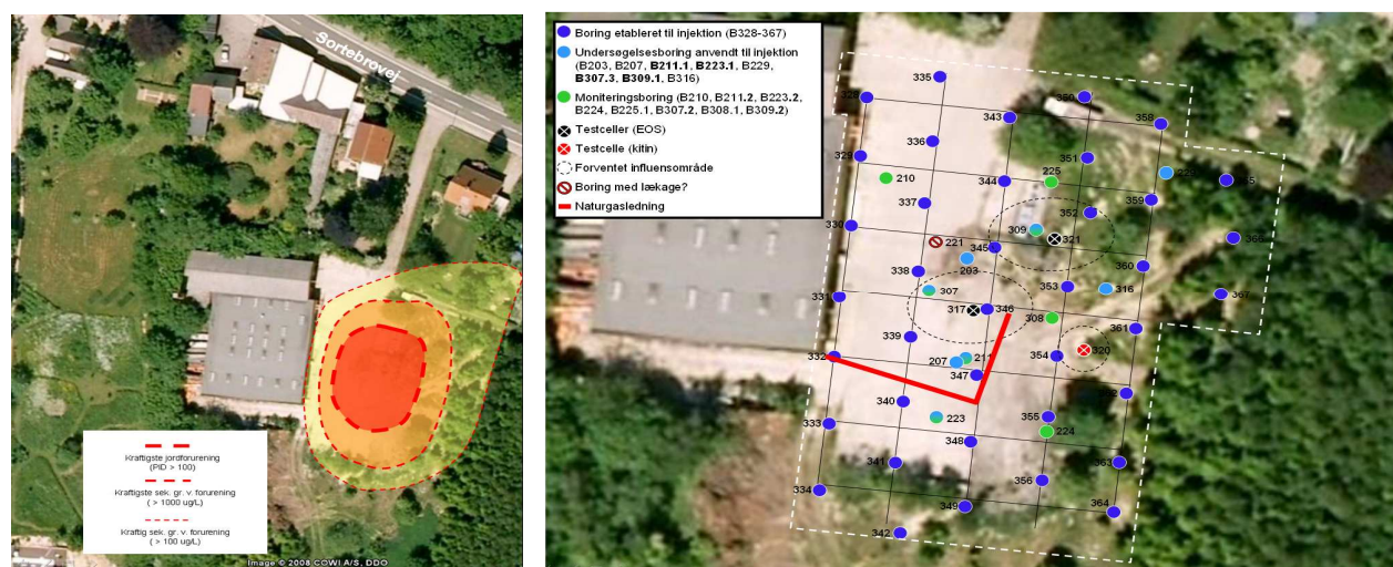
FIGURE 1. Sortebrovej site. TCE-contamination and network of injection wells for substrate and bioaugmentation culture injection in clay till.
