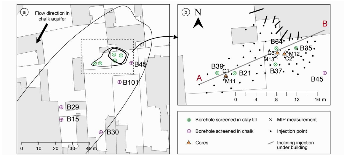
FIGURE 2. Gl. Kongevej site. TCE-contamination and network of injection points for substrate and bioaugmentation culture in source and plume areas in clay till. Modified from Damgaard et al. (2012).
