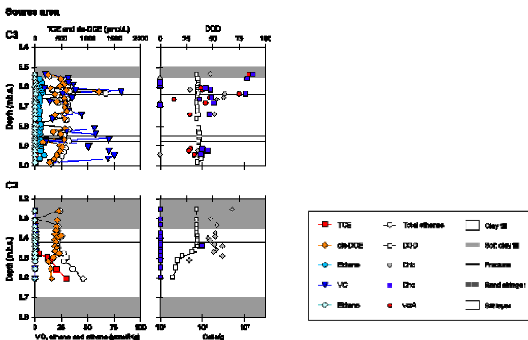
FIGURE 4. Gl. Kongevej site. Example core sections from the source zone illustrating sequential dechlorination and microbial composition. Modified from Damgaard (2012).
