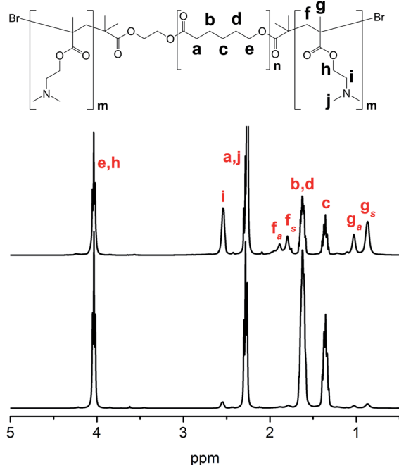
Fig. 2 ^1\text{H-NMR} spectra of the two triblocks PDMAEMA- b -PCL- b -PDMAEMA ( ABA , top) and PCL- b -PDMAEMA- b -PCL ( BAB , bottom) in \text{CDCl}_3 . Notations a and s added to f and g refer to tacticity; atactic and syndiotactic, respectively.
